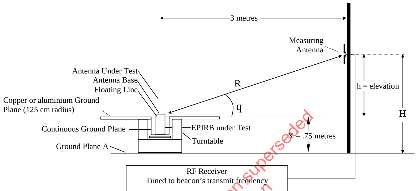
Figure B.4: Test Configuration for “EPIRB-like” Devices (i.e. beacons designed to operate while floating in water)
