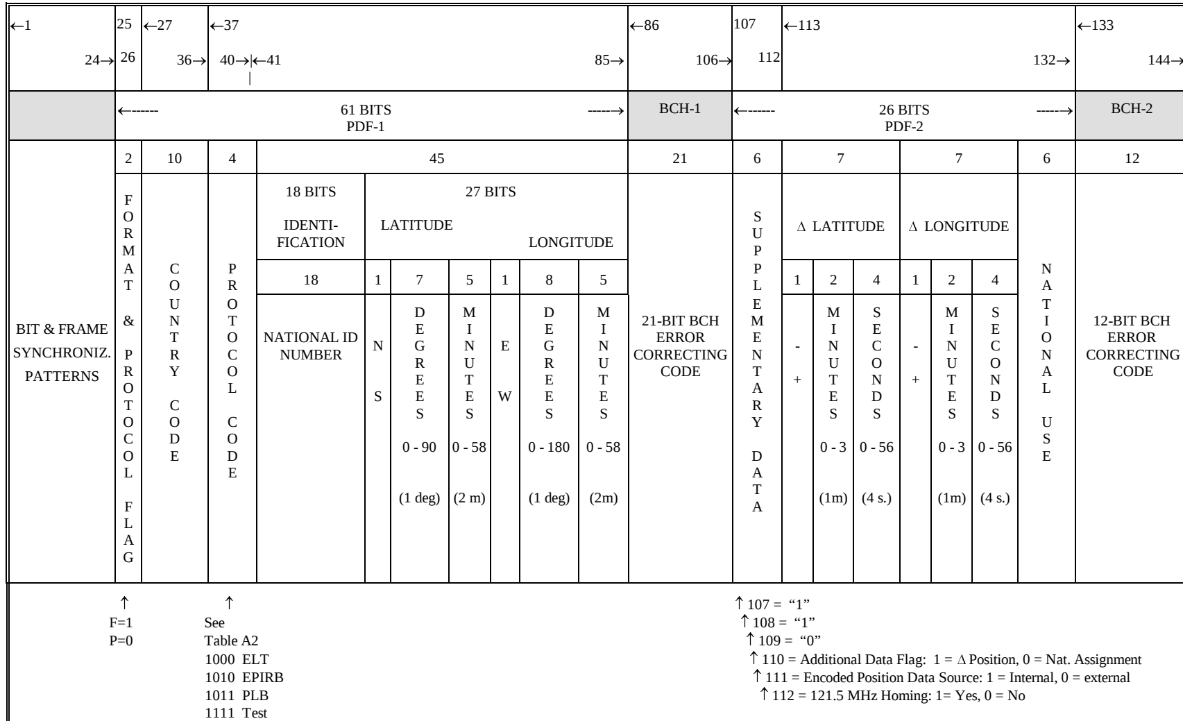
Figure A9: National Location Protocol
