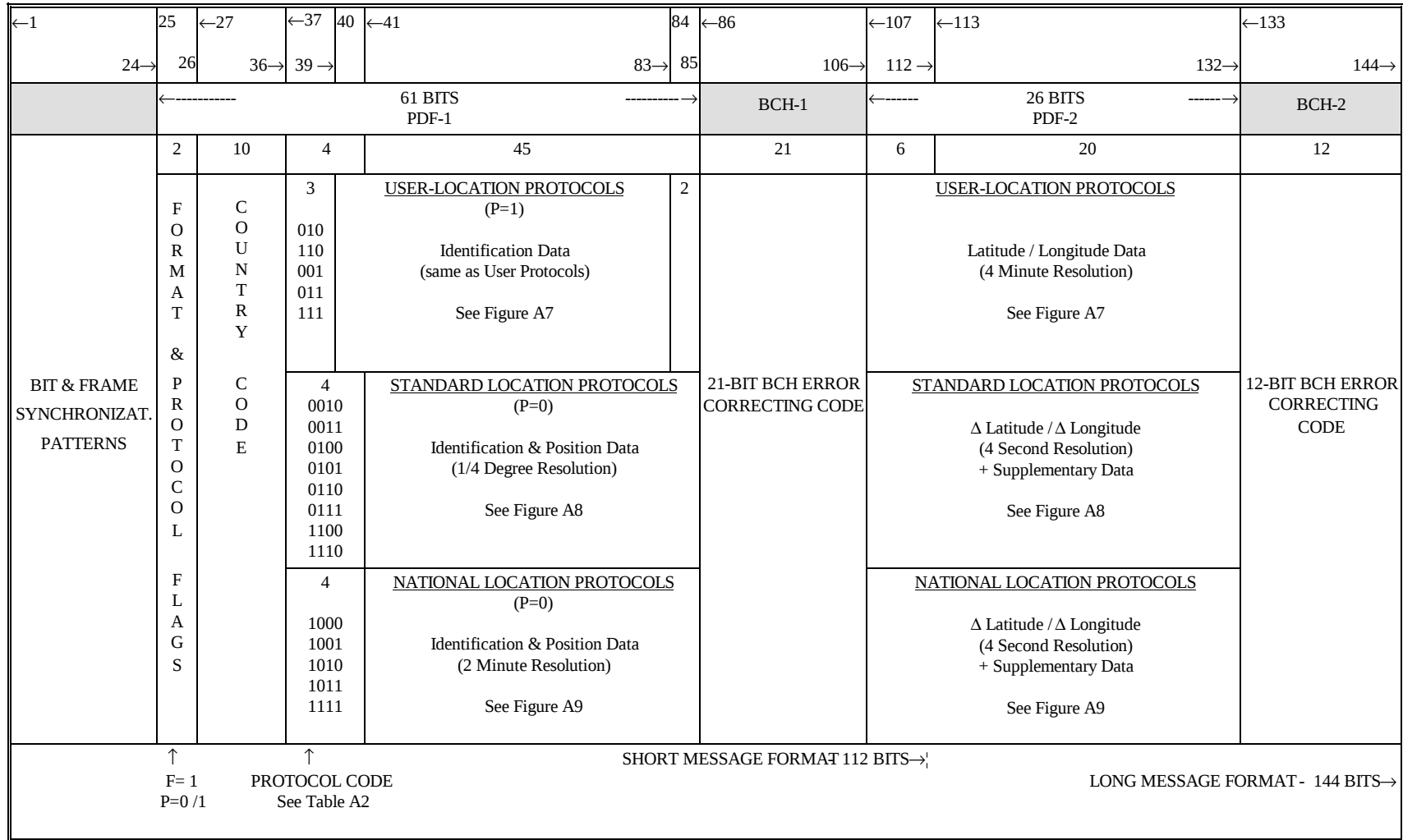
Figure A6: General Format of Long Message for Location Protocols
