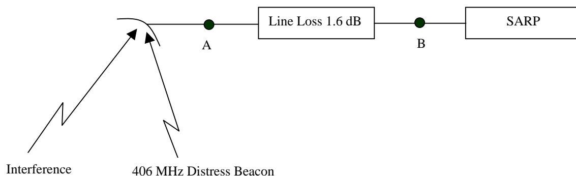
Figure E-B.1: Cospas 406 MHz SARP with Uplink Interference
