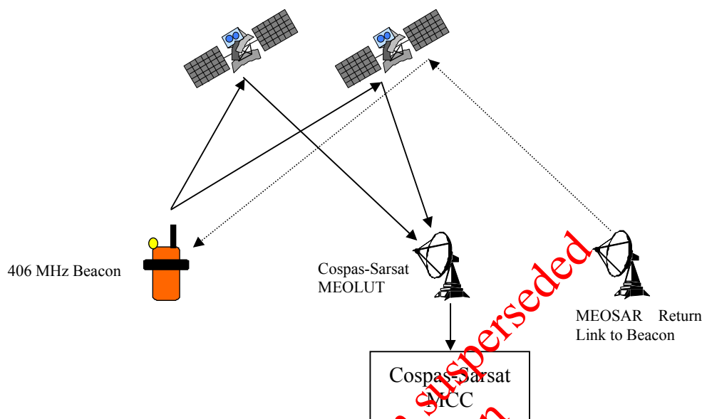
Figure 2.1: MEOSAR System Concept of Operations
