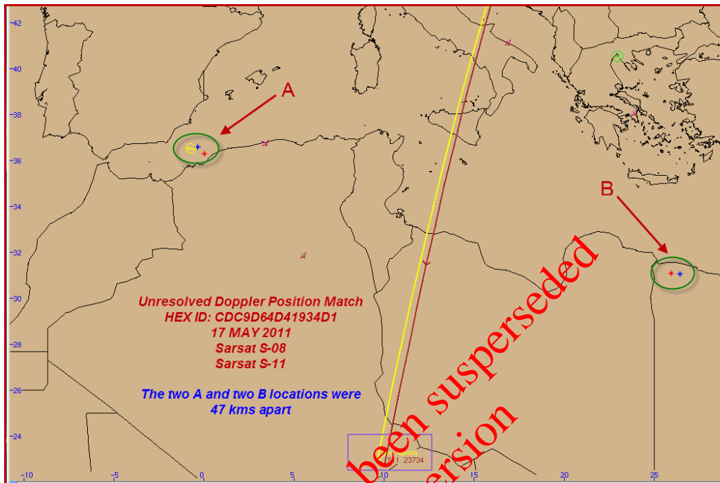
Figure 6.15: Unresolved Doppler Position Match
