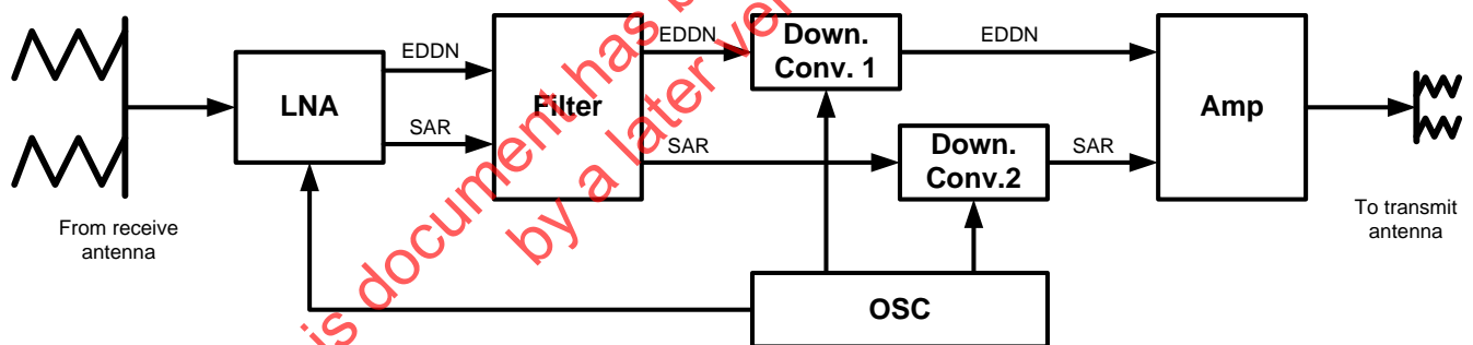
Figure 7.1: Louch-5A Combined SAR and EDDN Transponder
