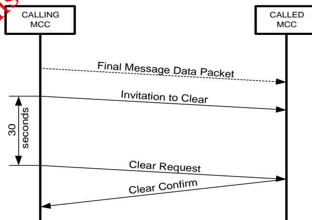
Figure E.3: Clearing Procedure if ITC Fails
