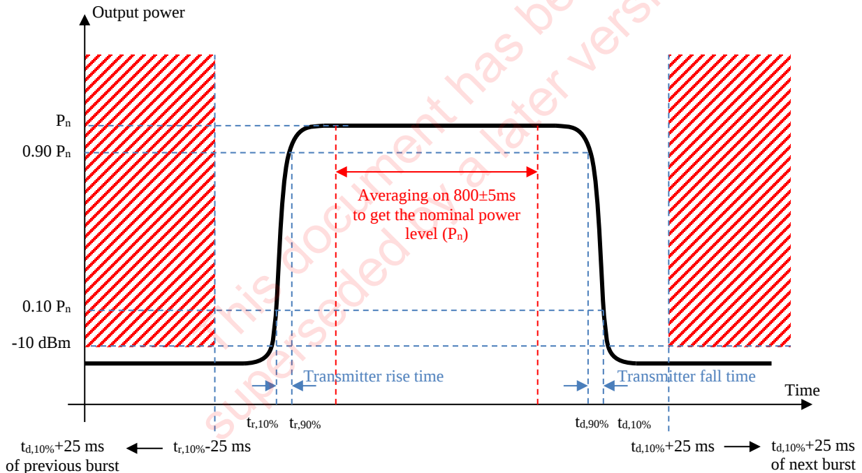
Figure B.6: Power Profile for Output Rise and Fall Time Measurement
