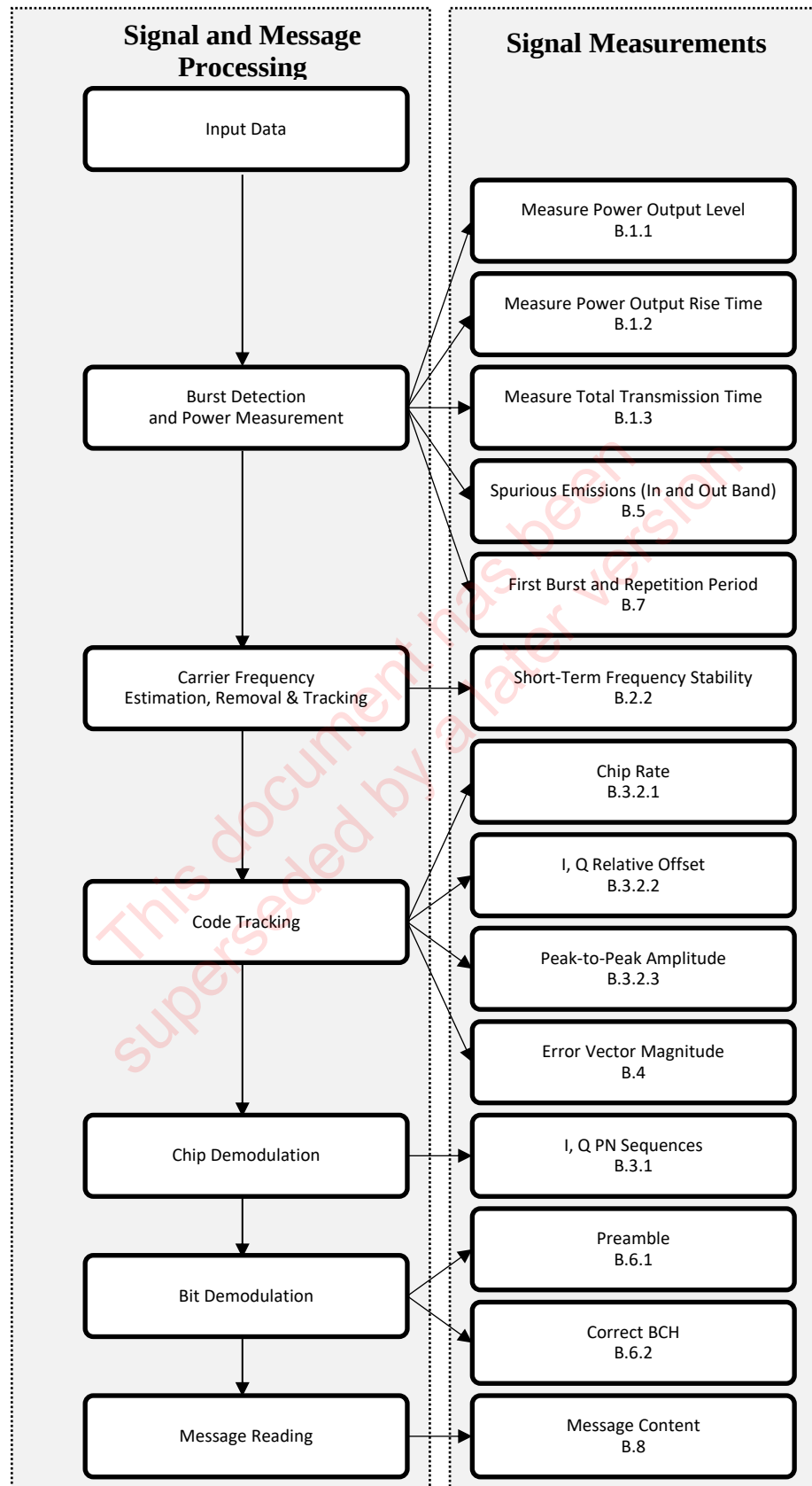
Figure B.1: Processing Steps
