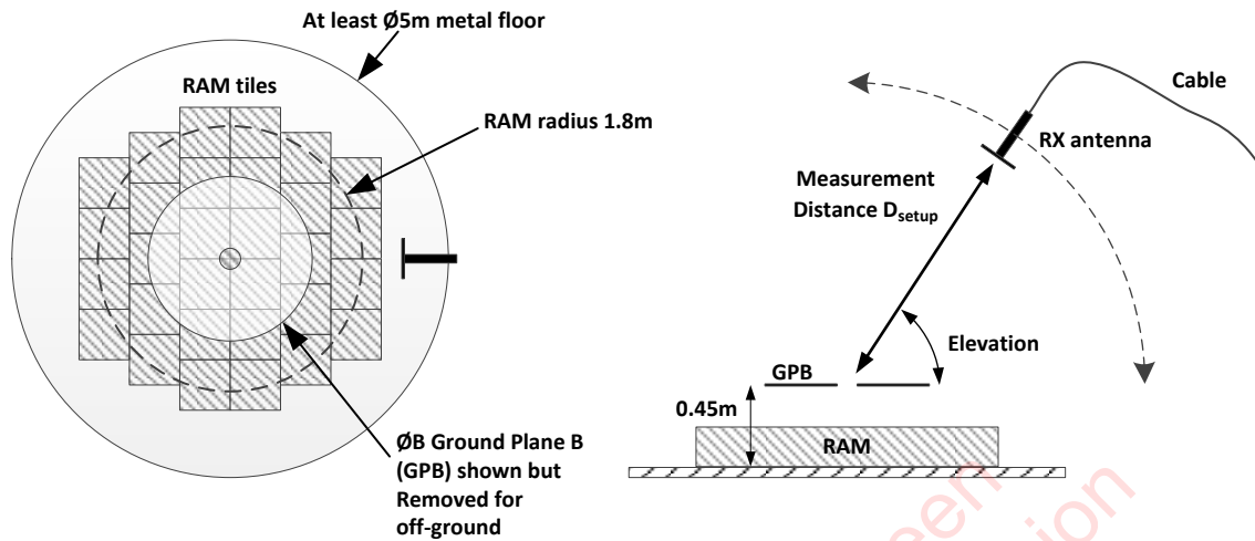
Figure B.14: Illustration of RAM zone and RX antenna path
