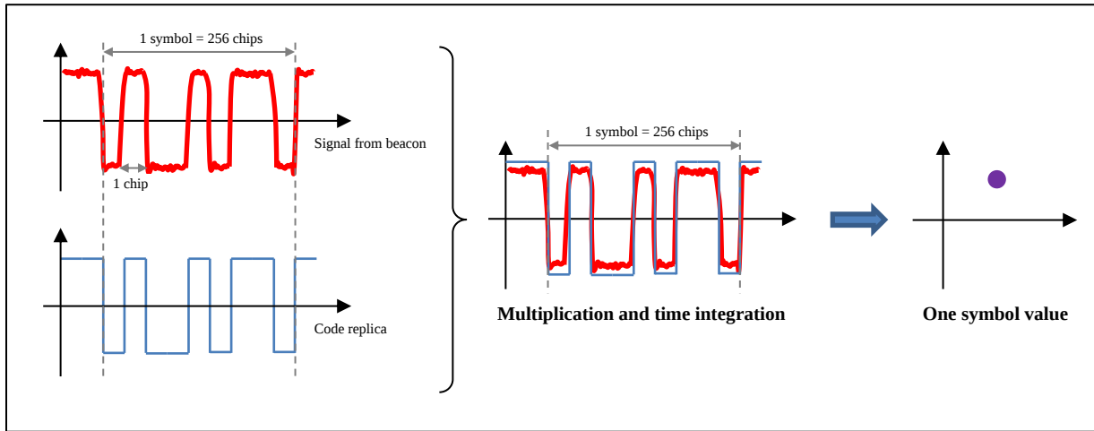
Figure B.11: Signal Integration and Symbol Values
