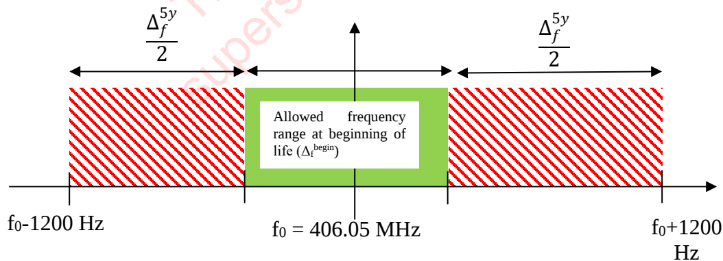
Figure B.8: Allowable Beginning-of-Life Frequency Range
