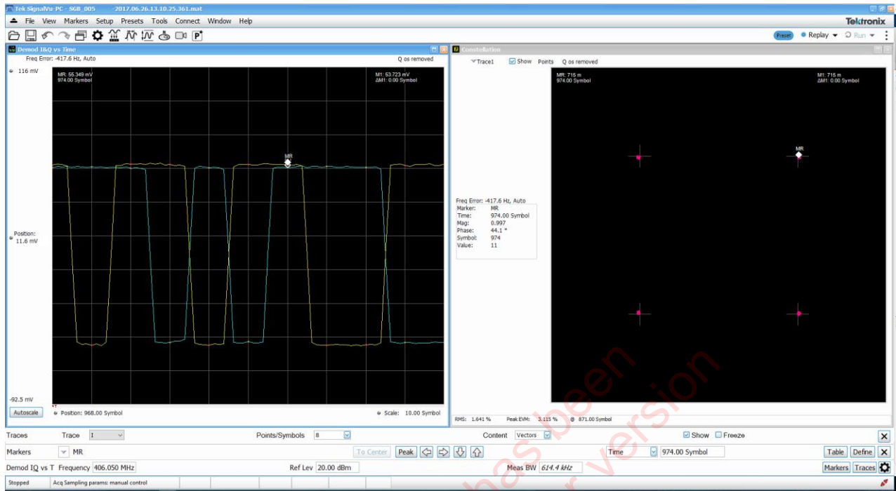
Figure B.12: Demodulation: Mapping from I/Q to Constellation
