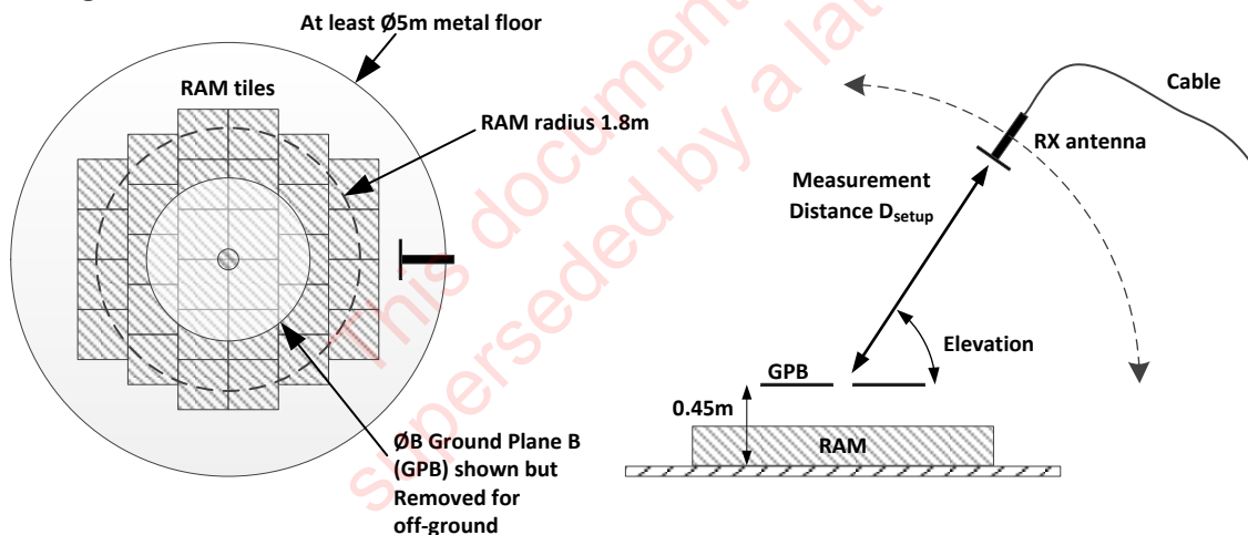
Figure B.13: Illustration of RAM zone and RX antenna path
