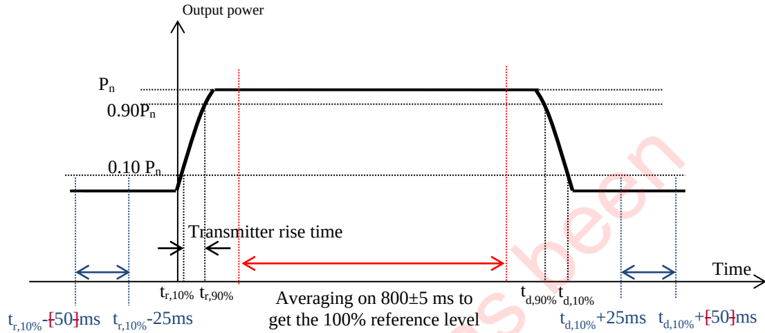
Figure B.6: Power Profile for Output Rise and Fall Time Measurement
