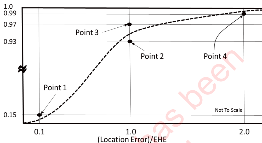
Figure C.1: (Location Error)/EHE Cumulative Distribution
