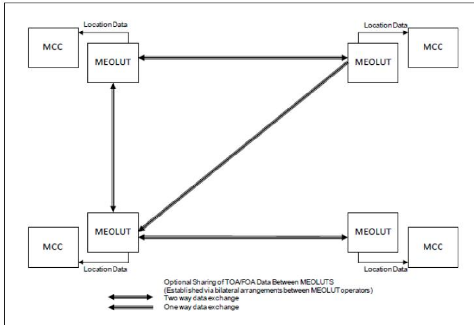
Figure C.1: Primary Topology for a MEOLUT Network: a Partial Mesh
