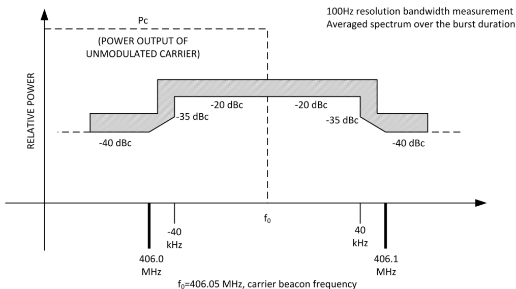
Figure 2-5: Spurious emission mask
