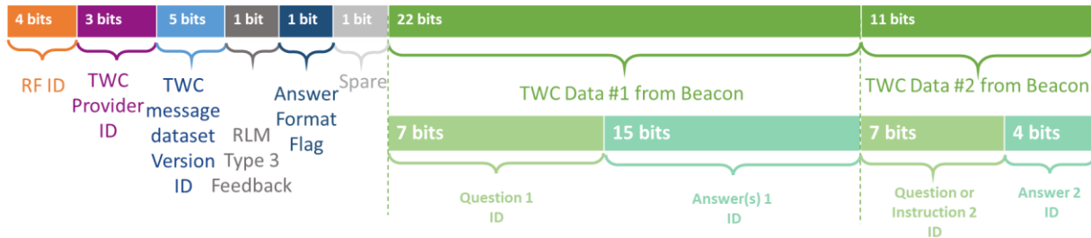
Figure 4-3: RF#4 bit assignment representation with the FLAM in the case where the bit 14 (Answer Format Flag) is 1 (Long)
