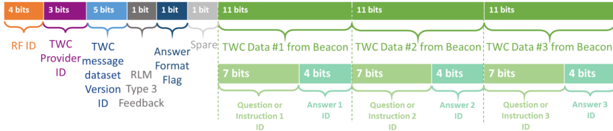
Figure 4-2: RF#4 bit assignment representation with the FLAM in the case where the bit 14 (Answer Format Flag) is 0 (Short)
