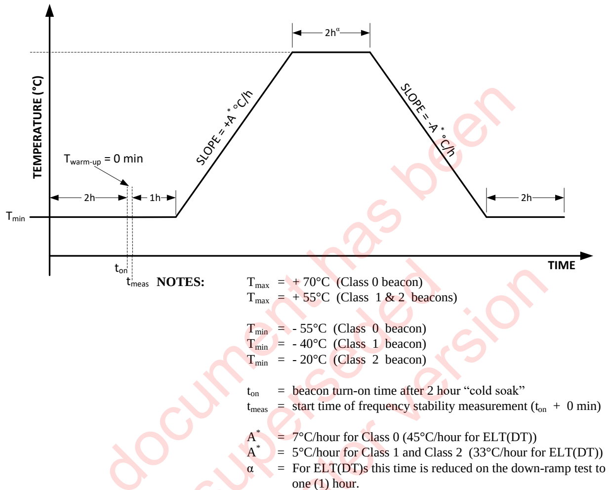
Figure 4-1: Temperature Gradient
