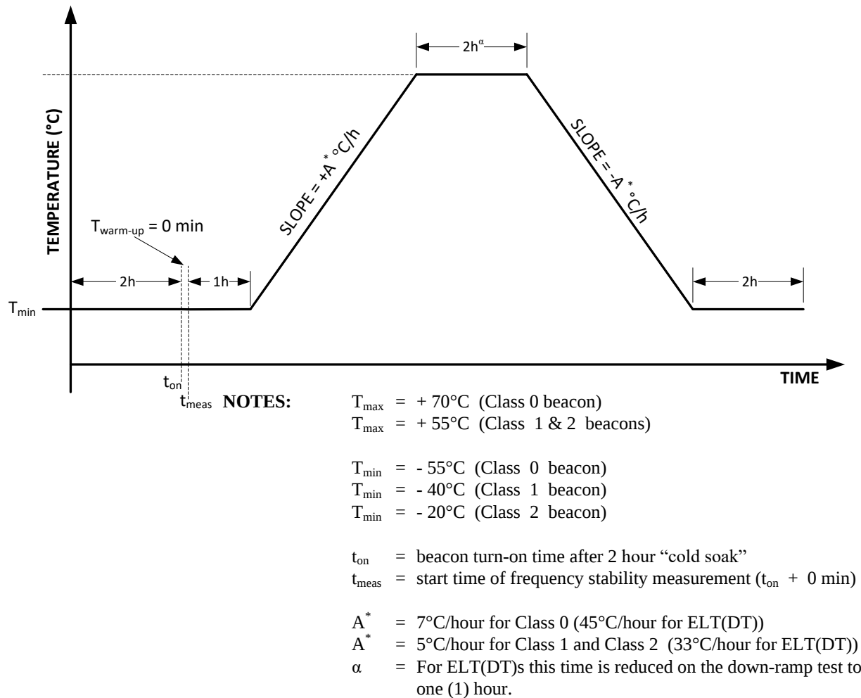
Figure 4-1: Temperature Gradient
