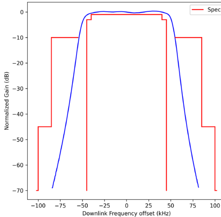
Figure 3.5: SAR/GPS Normalized Gain vs Downlink Frequency Offset
