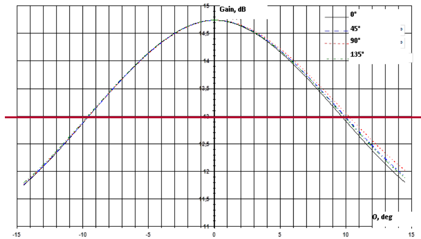
Figure 5.8: SAR Repeater Transmitting Antenna Gain (Four Cross-Sections)
