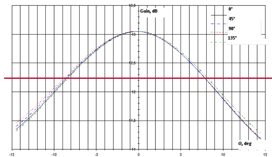
Figure 5.7: Glonass-K SAR Repeater Receiving Antenna Gain (Four Cross-Sections)
