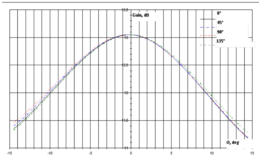
Figure 5.5: SAR Repeater Receiving Antenna Gain (Four Cross-Sections)
