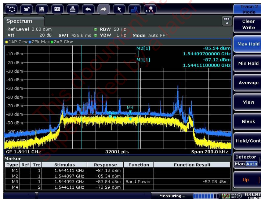
Figure 4.3: Galileo SAR Repeater L-Band Downlink Normal Band (90 kHz) Signal Spectrum
