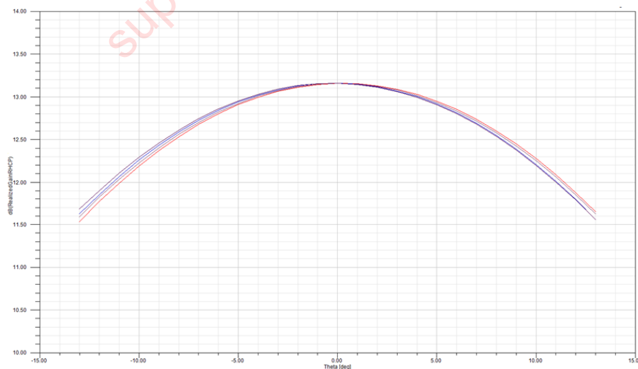
Figure 6.5: SAR/BDS Rx Antenna Gain (Four Cross-Sections)
