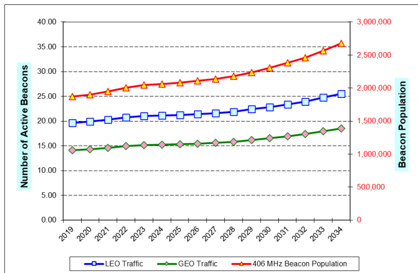
Figure G.4: LEOSAR and GEOSAR Beacon Message Traffic Forecast (Peak Traffic – 2025 model parameters/2024 population and traffic data)
