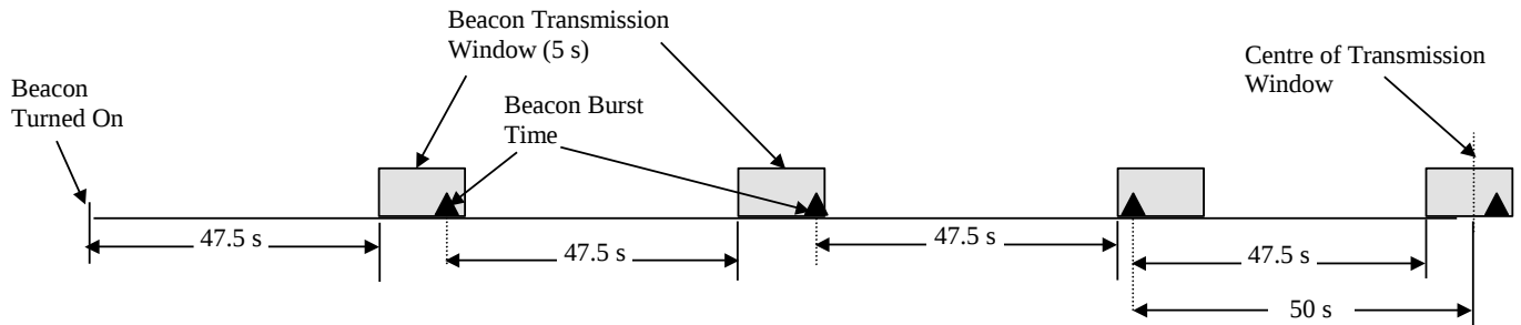
Figure D-D.3: C/S T.001 Specification Transmission Times
