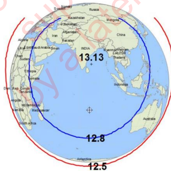
Figure 4-11: INSAT-3DS SASR 406.05 MHz Receive Antenna Contour Pattern
