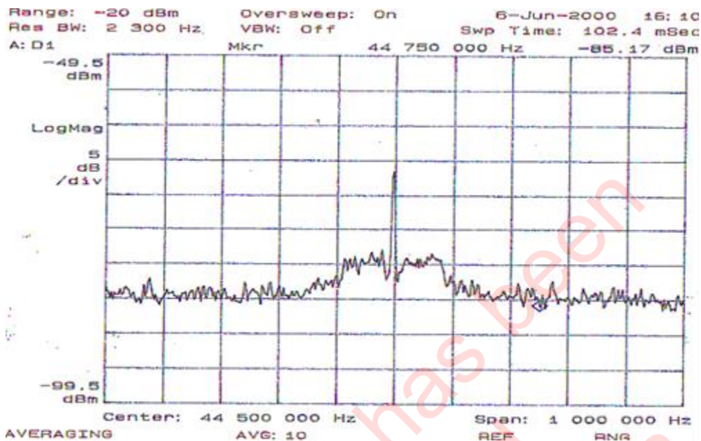
Figure 3-4: GOES (15 and Earlier) L-Band Transmitter Output Spectral Occupancy
