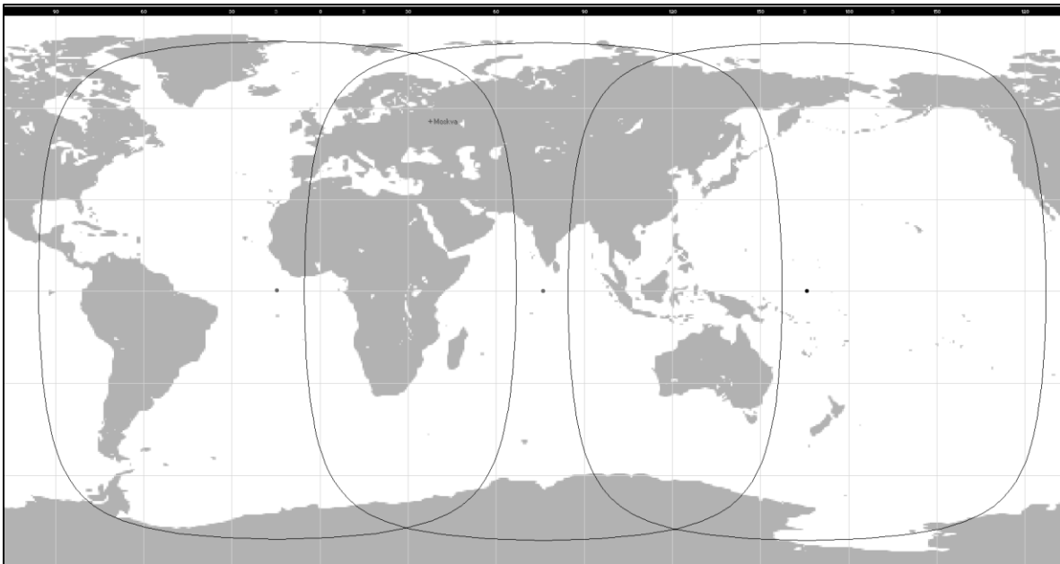
Figure 5-6: Electro-L 0° Elevation Angle Footprint (Electro- L No 2, 3 and 4)
