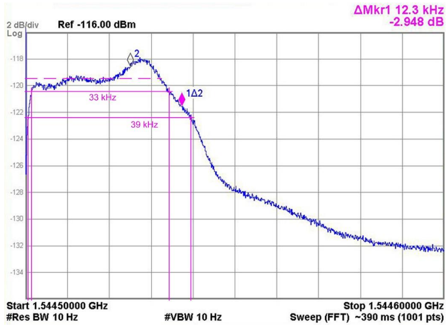
Figure 5-7: Electro-L SAR Receiver Bandpass Filter Amplitude-Frequency Response (Linear Phase Modulation Repeater NB Mode)
