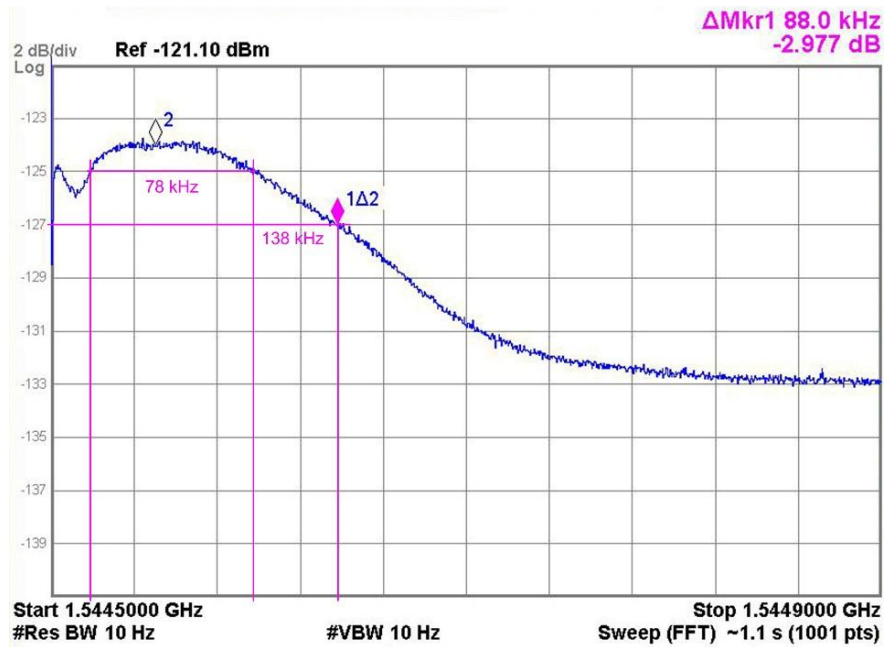
Figure 5-8: Electro-L SAR Receiver Bandpass Filter Amplitude-Frequency Response (Linear Phase Modulation Repeater WB Mode)
