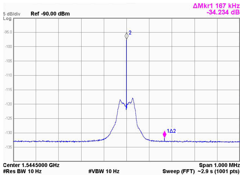
Figure 5-4: Spectrum Occupancy of Downlink Signal in NB Mode Spanned 1 MHz Around 1544.5 MHz
