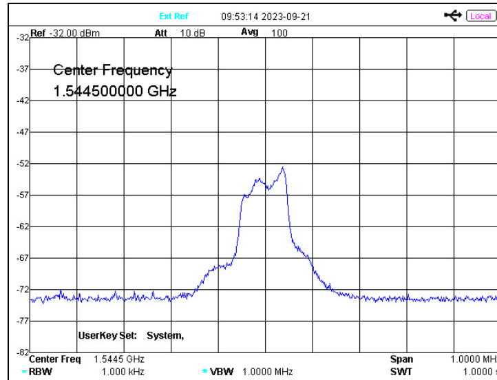
Figure 5-5: Spectrum Occupancy of Downlink Signal Centred at 1544.5 MHz. Electro-L No.4
