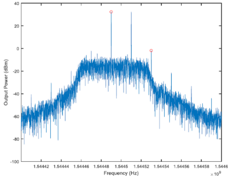
Figure 8-2: MTG Repeater Output Spectrum (Narrowband Mode)
