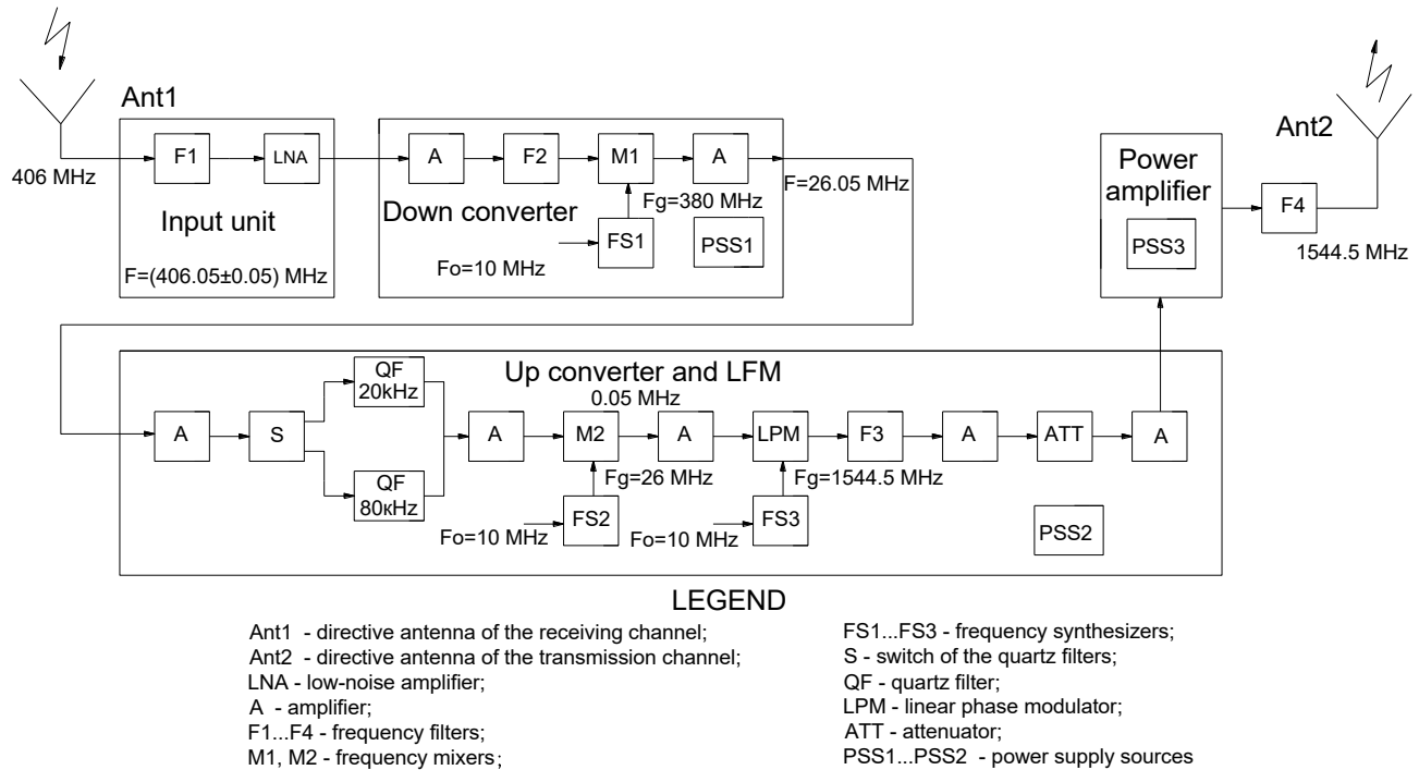
Figure 5-1: Electro-L SAR Functional Diagram (Linear Phase Modulation Repeater)
