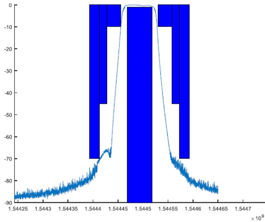
Figure 8-4: MTG SAR Repeater Narrowband Filter Performance
