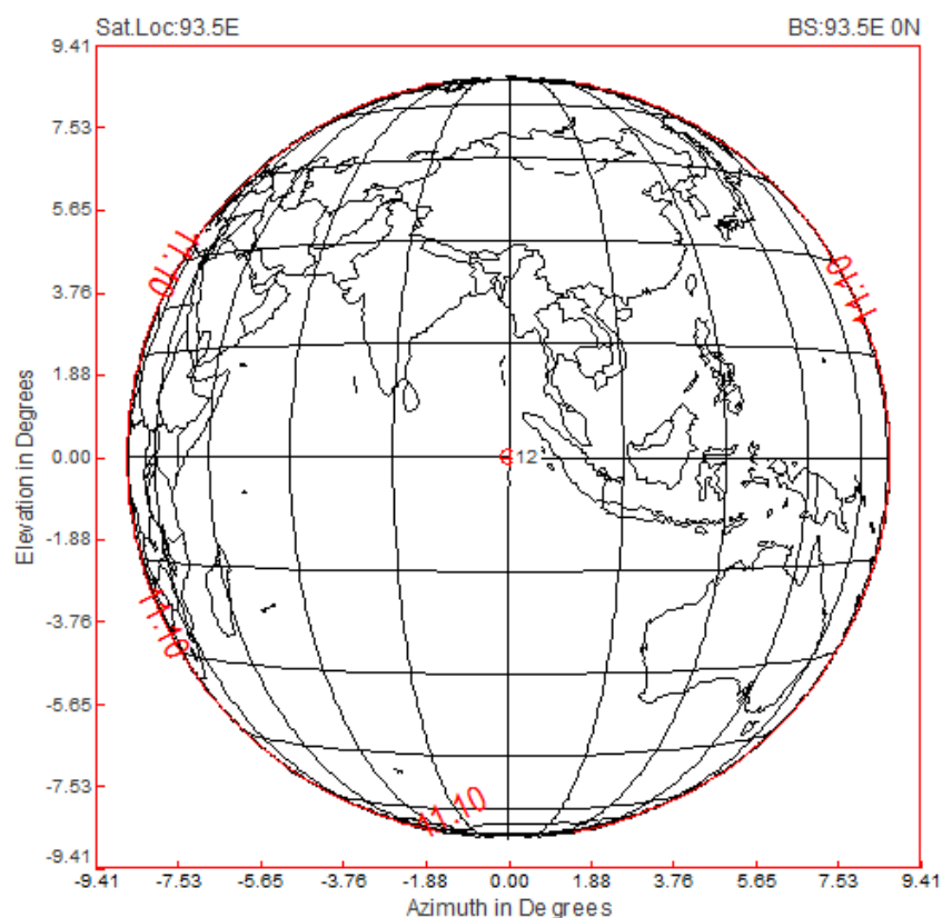
Figure 4-10: GSAT-17 SAR 406.05 MHz Receive Antenna Contour Pattern
