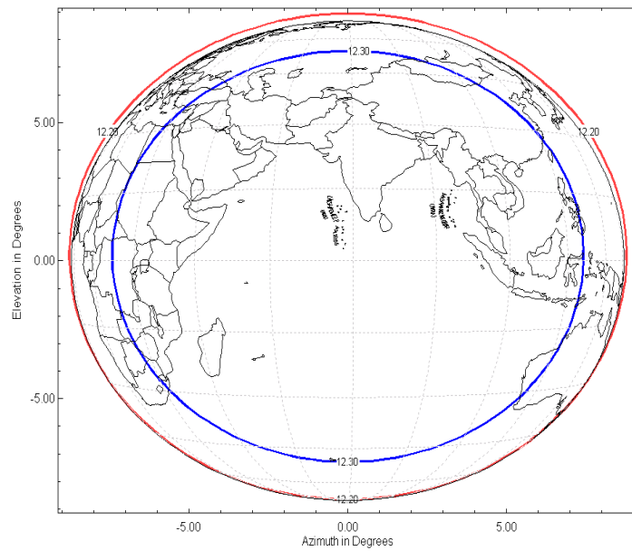
Figure 4-9: INSAT-3DR SASR 406.05 MHz Receive Antenna Contour Pattern
