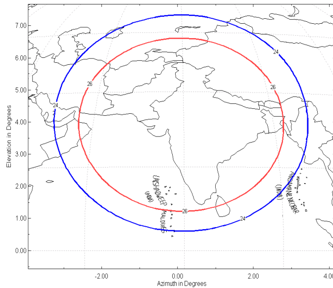
Figure 4-13: INSAT-3DR Transmit Antenna Contour Pattern
