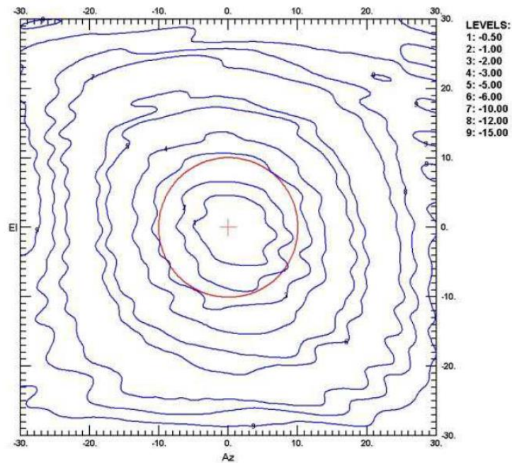
Figure 8-7: MTG L-Band Antenna Co-Polar Amplitude Pattern (Antenna Gain in dB Relative to the Peak Gain of 14.2 dB; Red Circle Shows the Earth)
