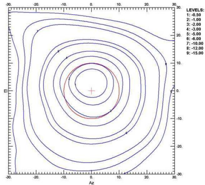
Figure 8-6: MTG UHF-Band Antenna Co-Polar Amplitude Pattern (Antenna Gain in dB Relative to the Peak Gain of 14.2 dB; Red Circle Shows the Earth)
