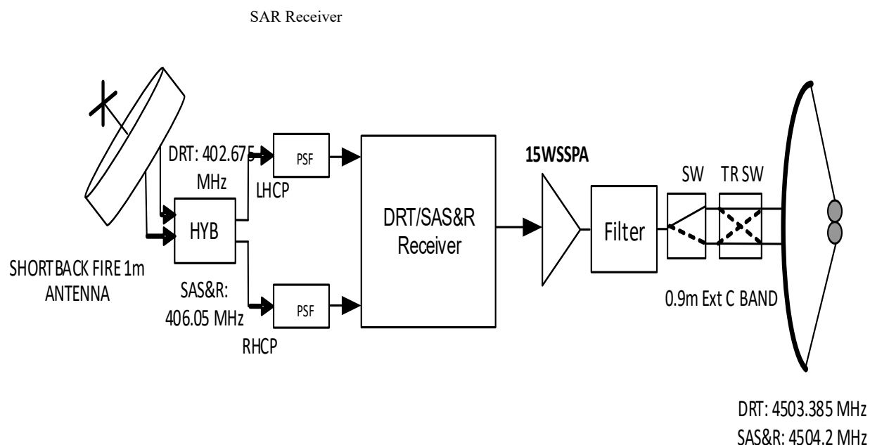
Figure 4-1: INSAT/GSAT SAR / DRT Repeater Functional Block Diagram
