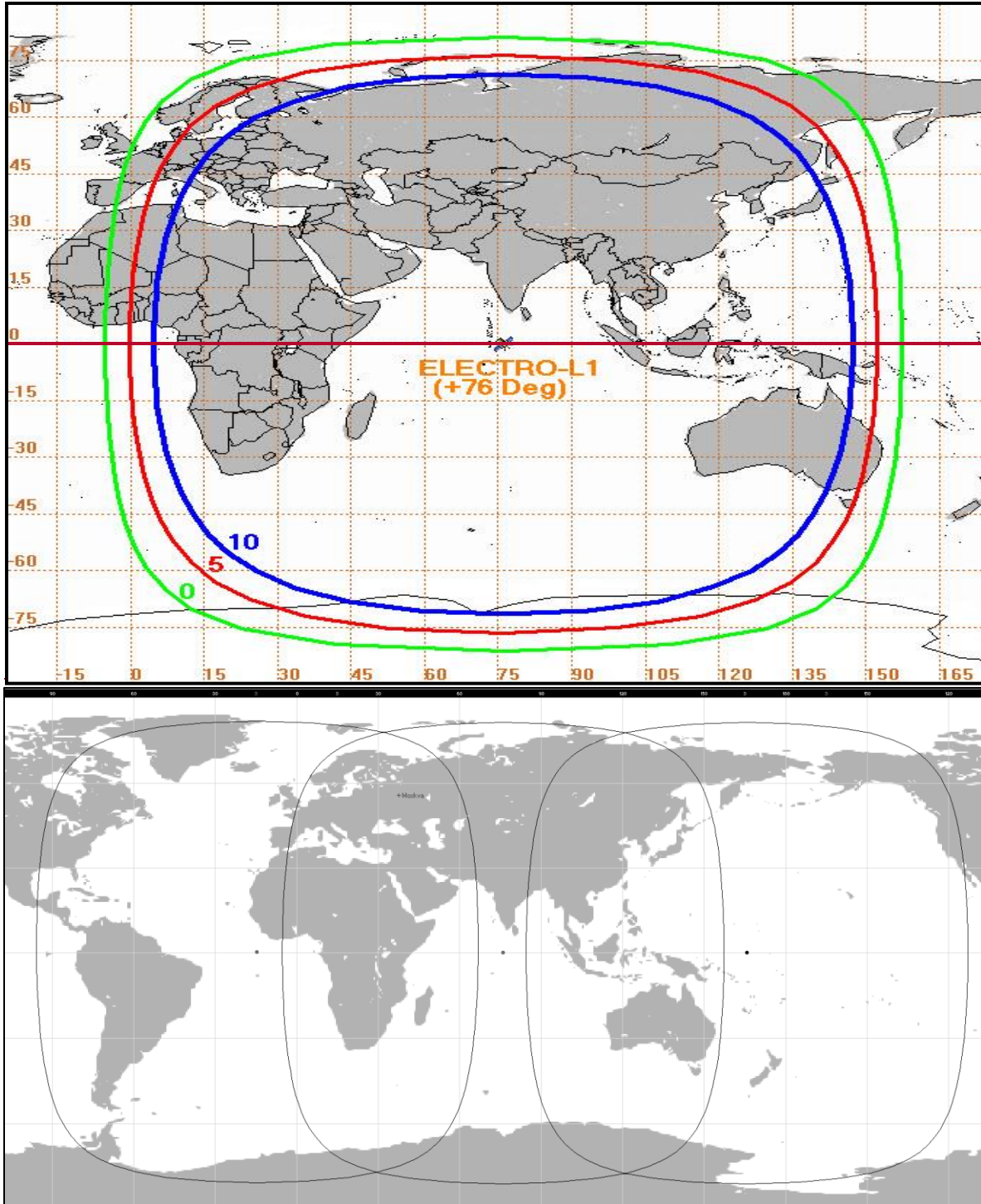
Figure 5-64: Electro-L1 0°, 5°, 10° Elevation Angle Footprint Coverage Contours (Electro- L No 2, 3 and 4)
