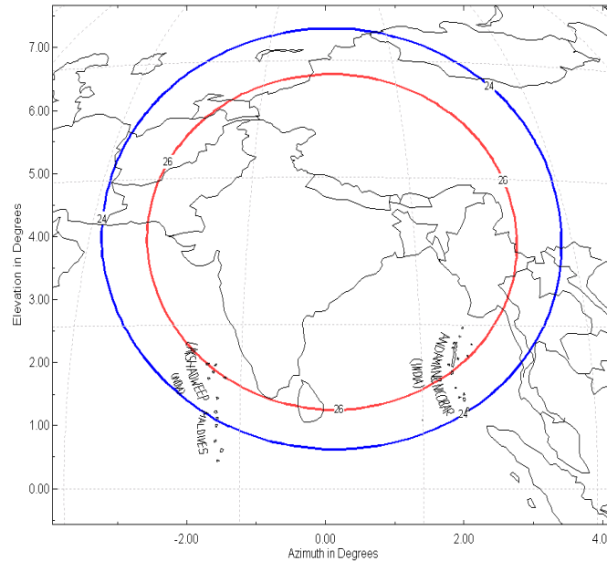
Figure 4-12: INSAT-3D Transmit Antenna Contour Pattern
