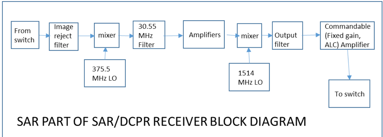
Figure 3-3: SAR Part of SAR/DCPR Receiver Block Diagram
