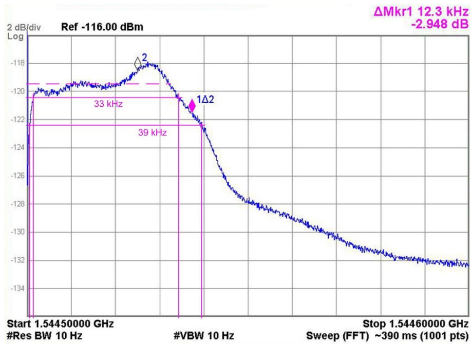
Figure 5-57: Electro-L1 SAR Receiver Bandpass Filter Amplitude-Frequency Response (Linear Phase Modulation Repeater in NB Mode)
