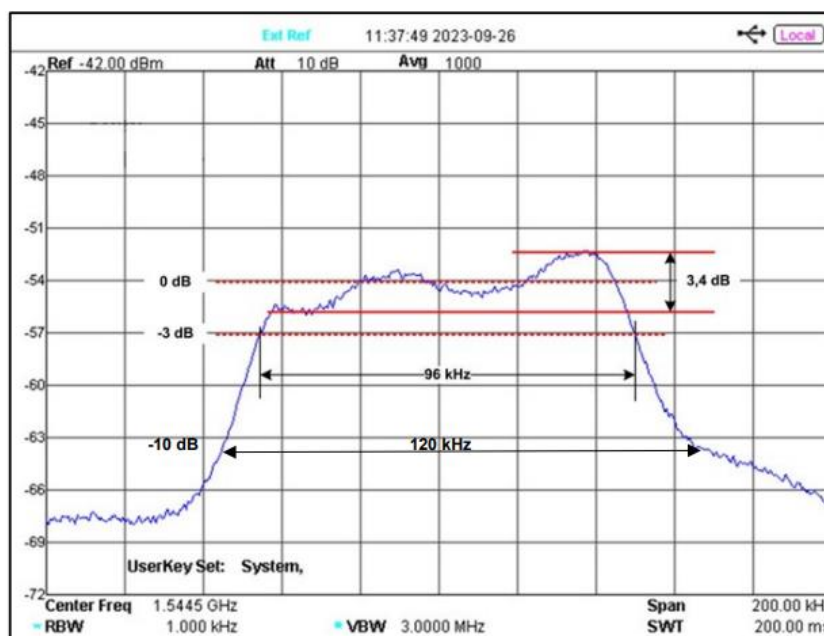
Figure 5-9: Electro-L SAR Receiver Bandpass Filter Amplitude-Frequency Response (Frequency Translation Repeater)
