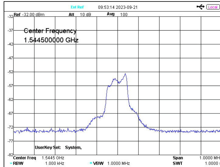
Figure 5-5: Spectrum Occupancy of Downlink Signal Centered at 1544.5 MHz. Electro-L No.4
