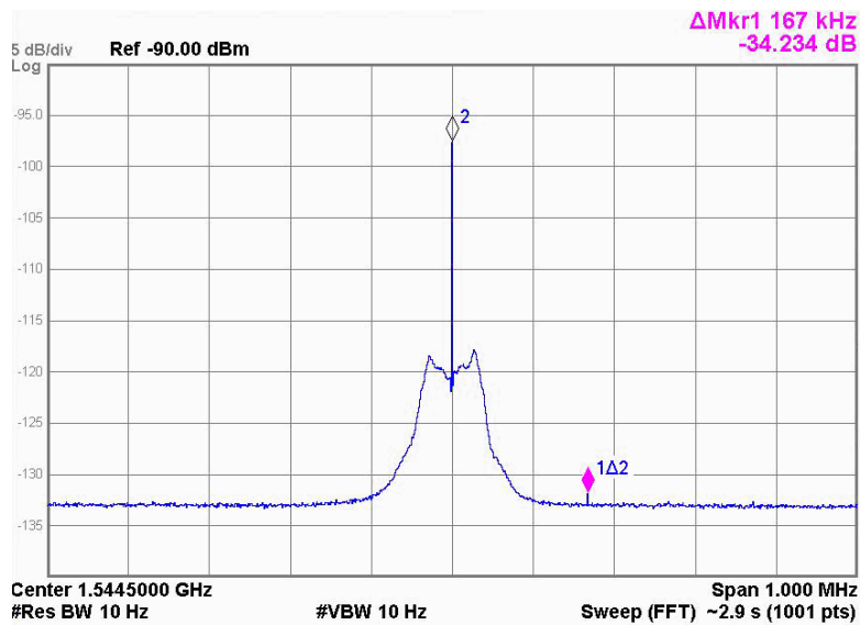
Figure 5-43: Spectrum Occupancy of Downlink Signal in NB Mode Spanned 1 MHz Around 1544.5 MHz
