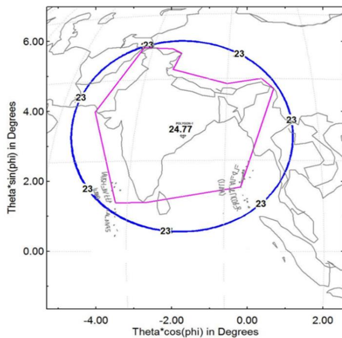
Figure 4-14: GSAT-17 Transmit Antenna Contour Pattern
