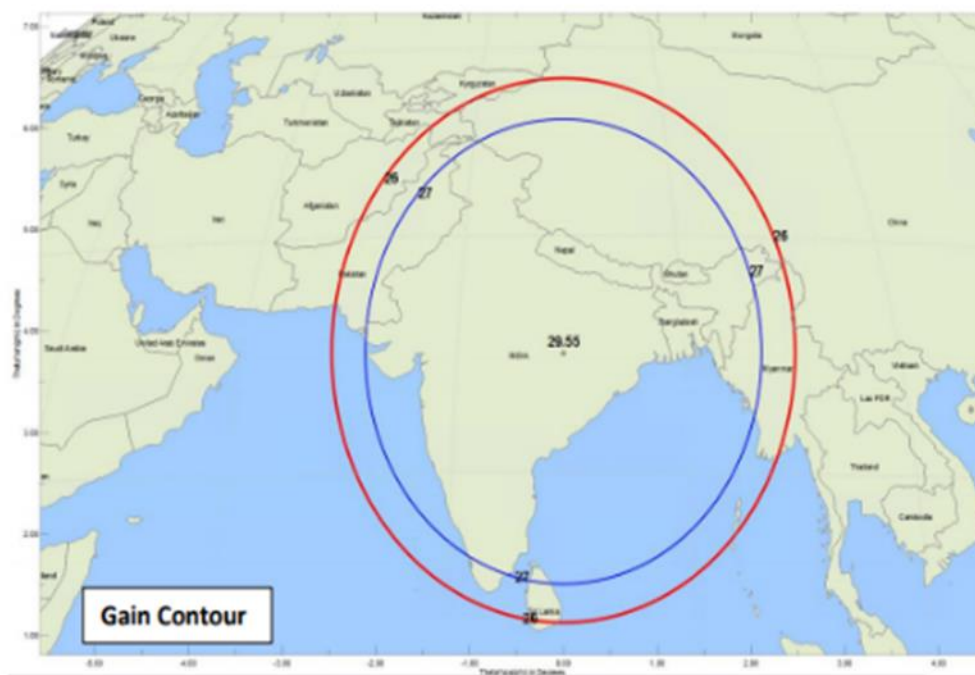
Figure 4-15: INSAT-3DS Transmit Antenna Contour Pattern
