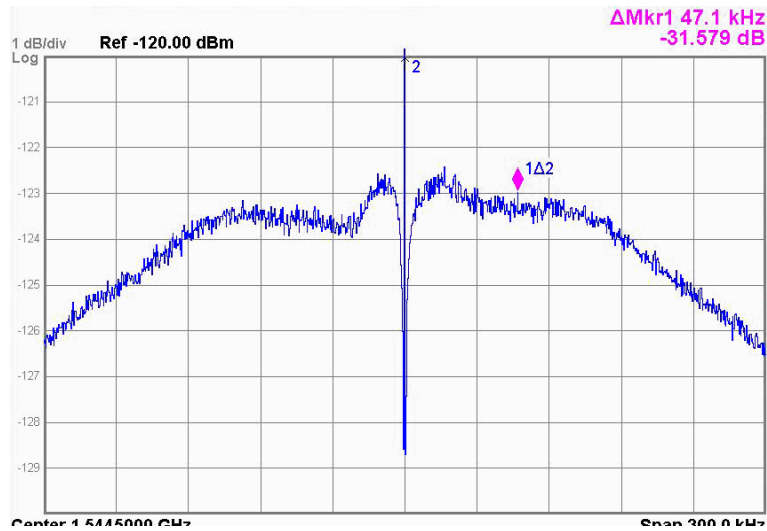
Figure 5-32: Spectrum Occupancy of Downlink Signal in WB Mode Spanned 300 kHz Around 1544.5 MHz
