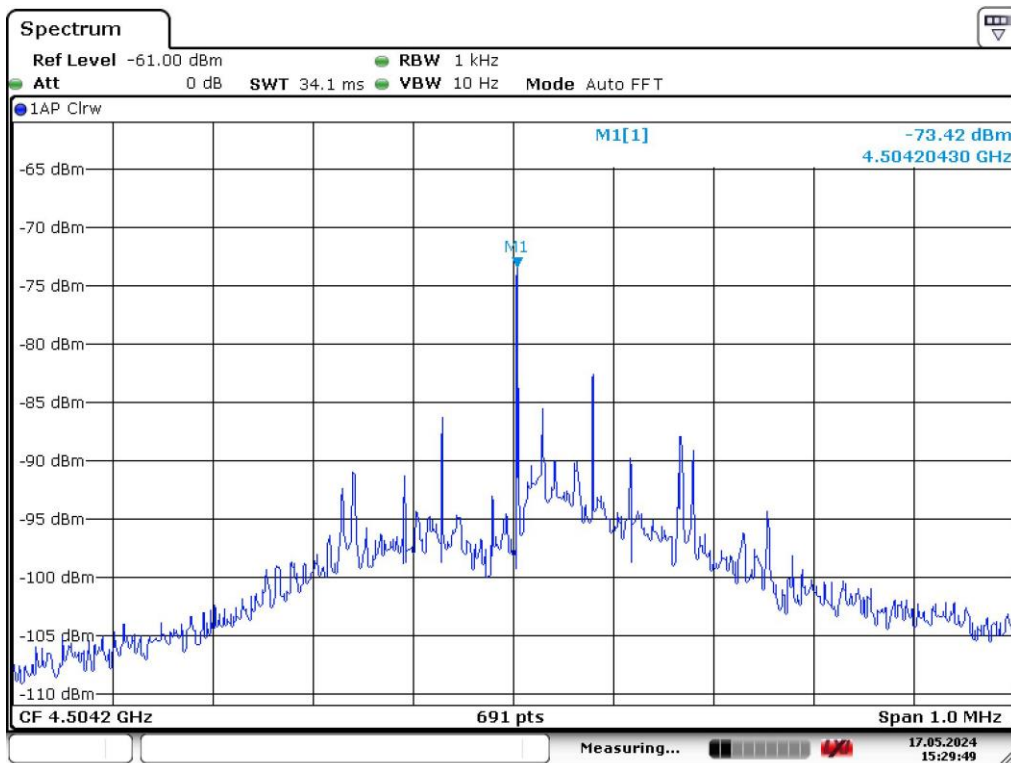
Figure 4-3: GSAT Transmitter Output Spectral Occupancy with No Test Signal
