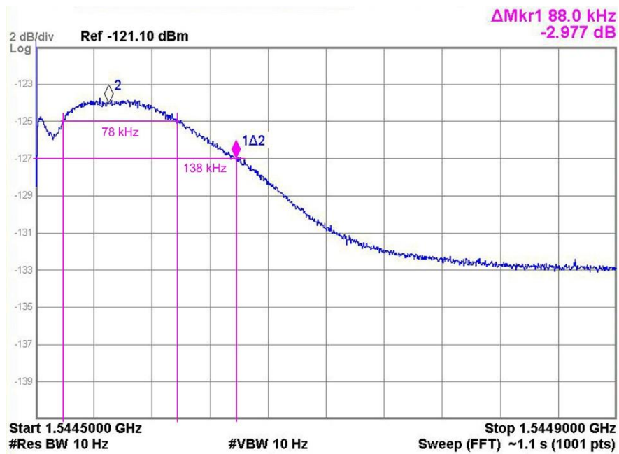
Figure 5-68: Electro-L1 SAR Receiver Bandpass Filter Amplitude-Frequency Response (Linear Phase Modulation Repeater in WB Mode)
