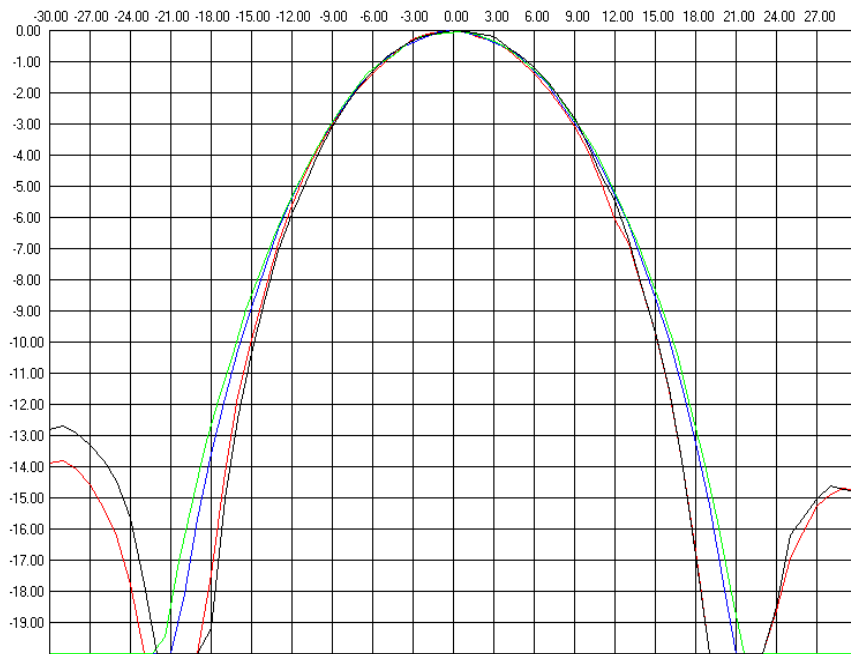
Figure 7-5: Louch-5A Transmit Antenna Pattern at 1544.5 MHz
