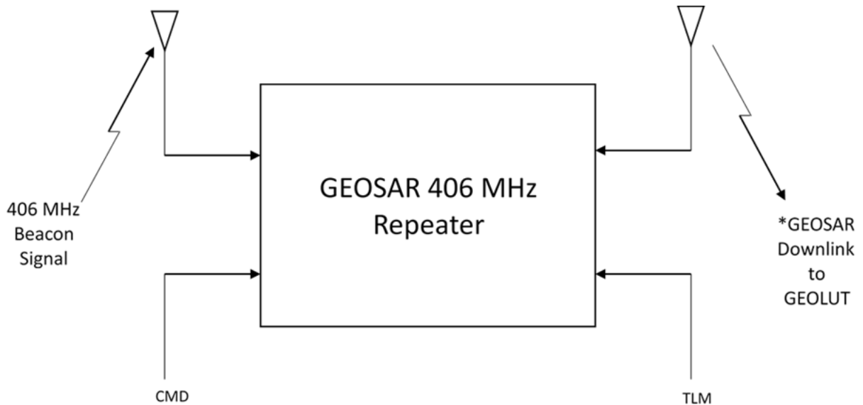
Figure 2-1: GEOSAR Payload Functional Diagram
