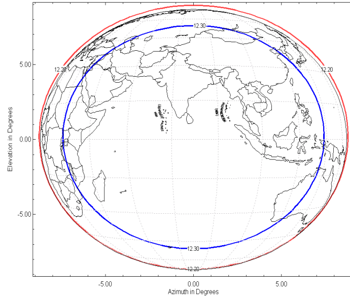
Figure 4-8: INSAT-3D SASR 406.05 MHz Receive Antenna Contour Pattern
