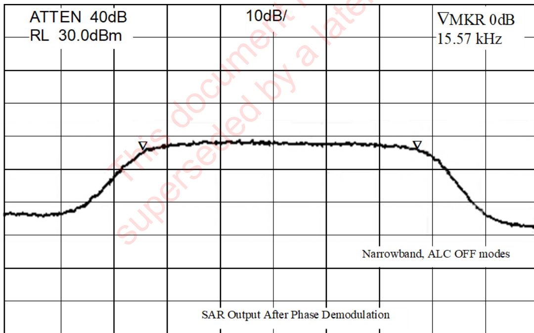
Figure 3-5: For all GOES up to GOES-15: Narrow Band Baseband Spectrum
