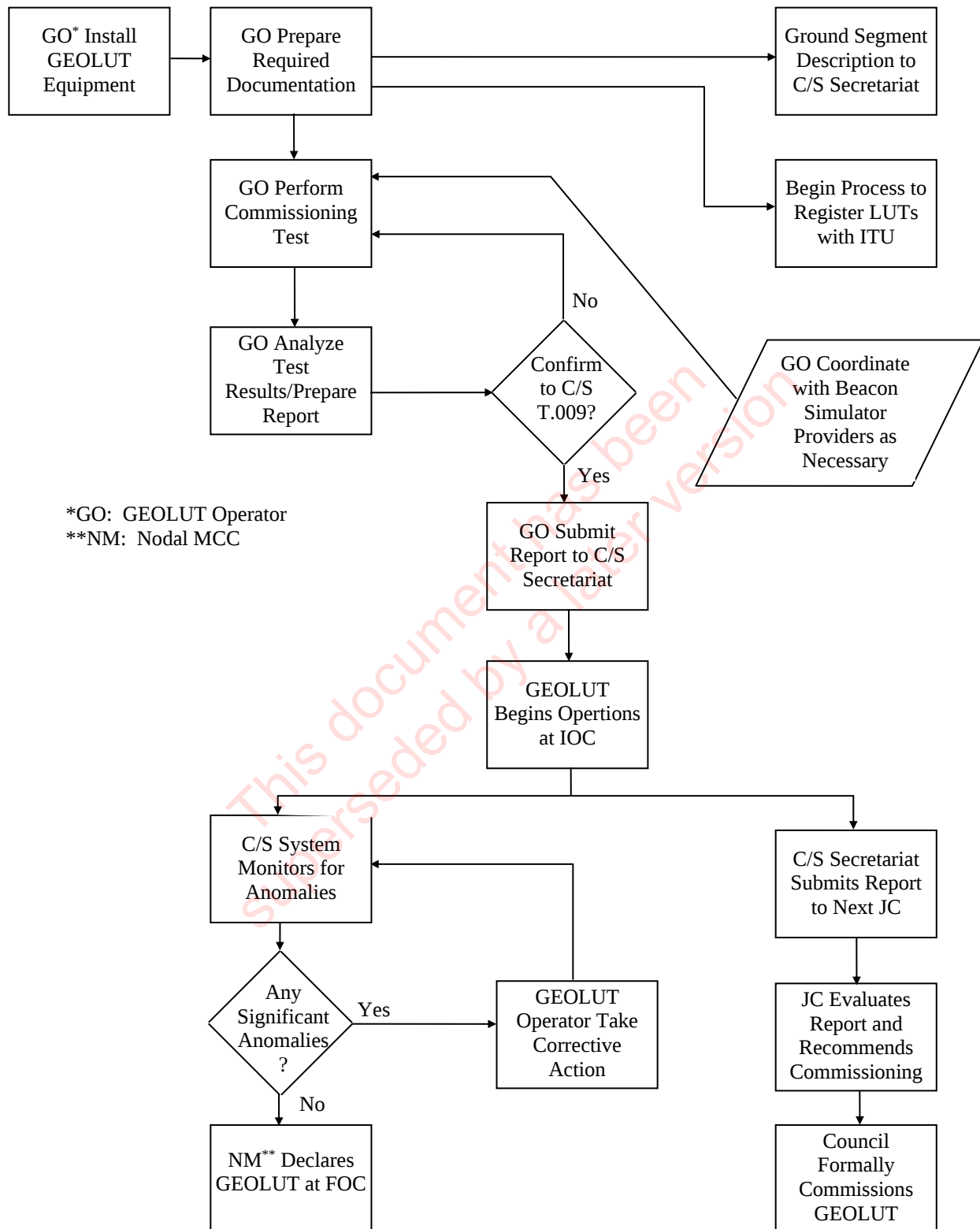
Figure G.1: Overview of GEOLUT Integration -END OF ANNEX G-
