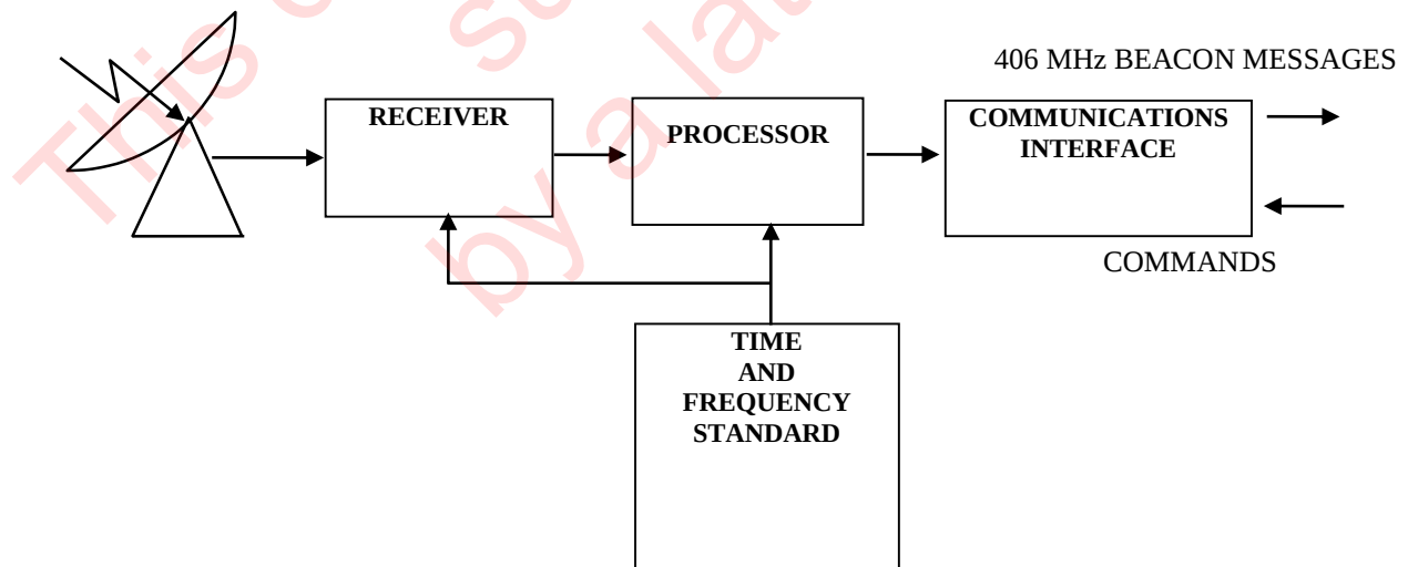
Figure 2.1: A Typical Cospas-Sarsat GEOLUT Functional Block Diagram
