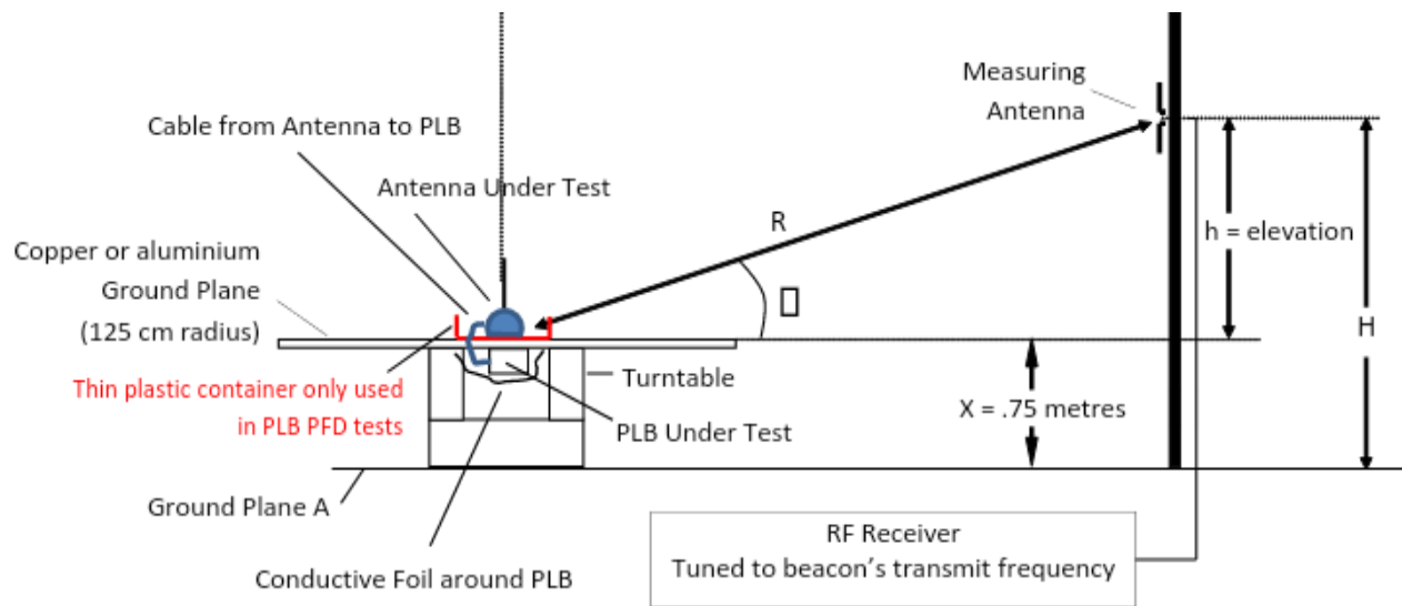
Figure B.2a: Test Configuration for PLBs on PFDs with Non-Integral Antennas
