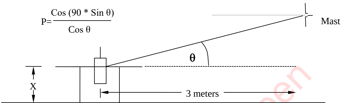
Figure B.8: Measuring Antenna NOT Perpendicular to the Direction of Propagation
