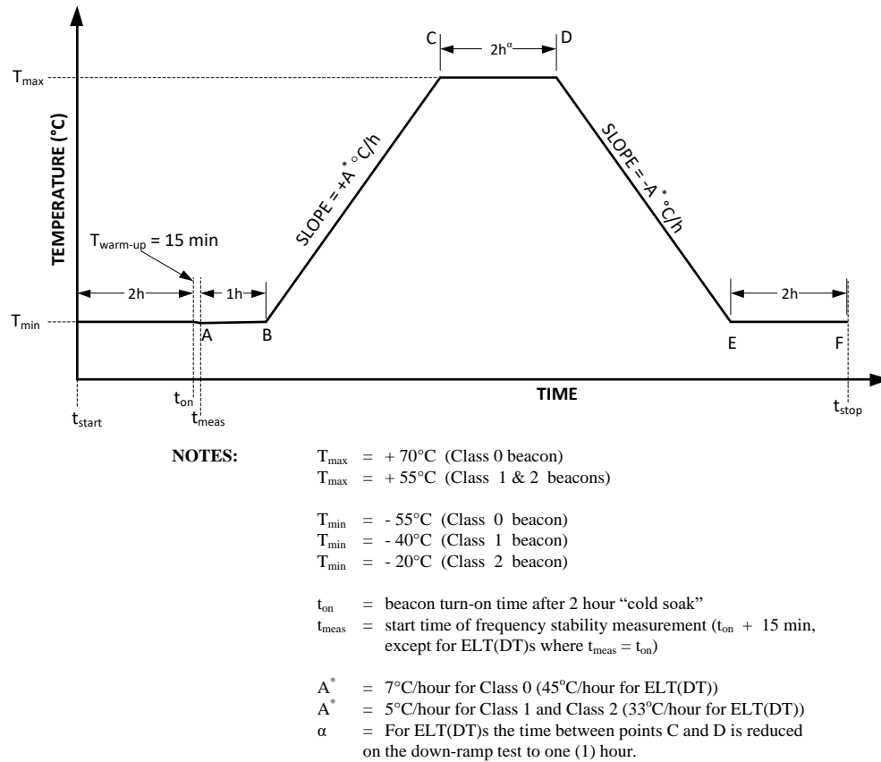
Figure A.1: Temperature Gradient Test Profile
