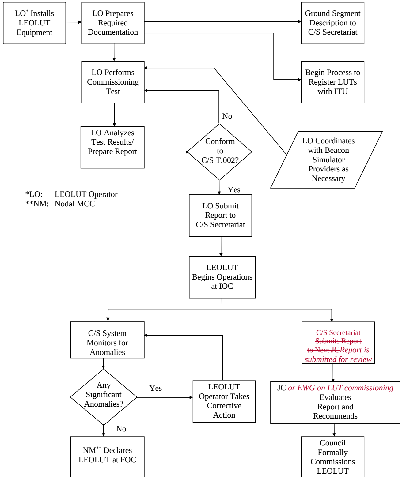
Figure G.1: Overview of LEOLUT Integration
