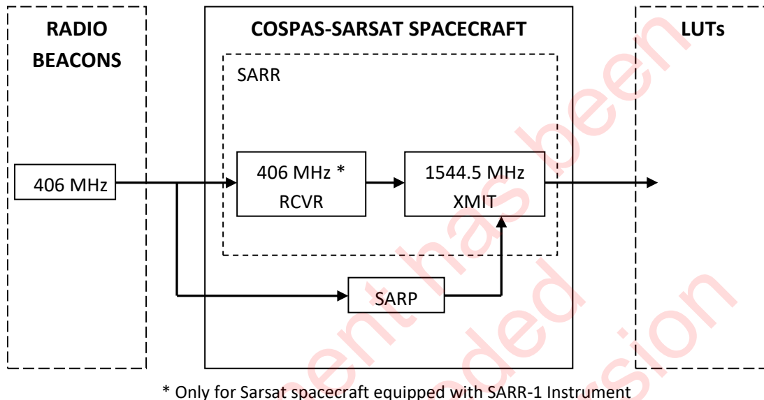
Figure 1.1: Cospas-Sarsat LEOSAR Space Segment
