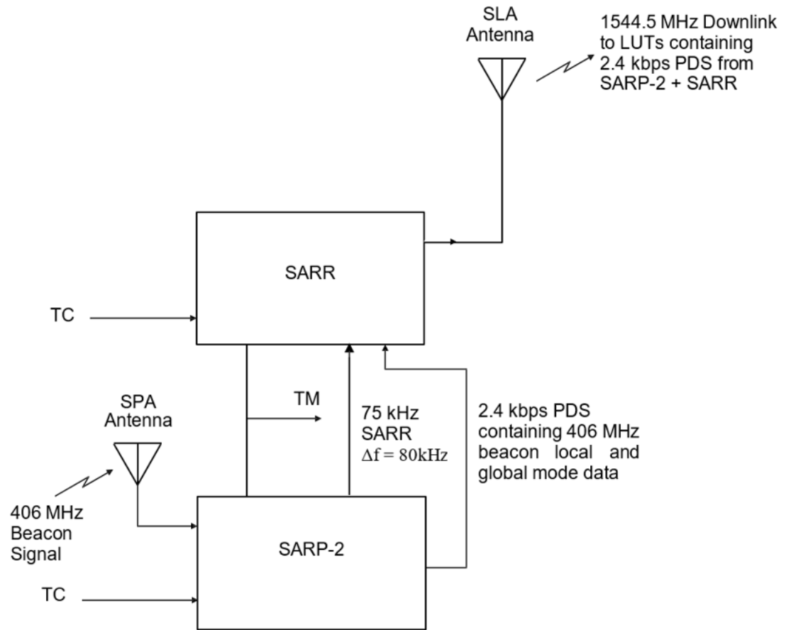
Figure 2-1: Cospas-Sarsat System Functional Diagram
