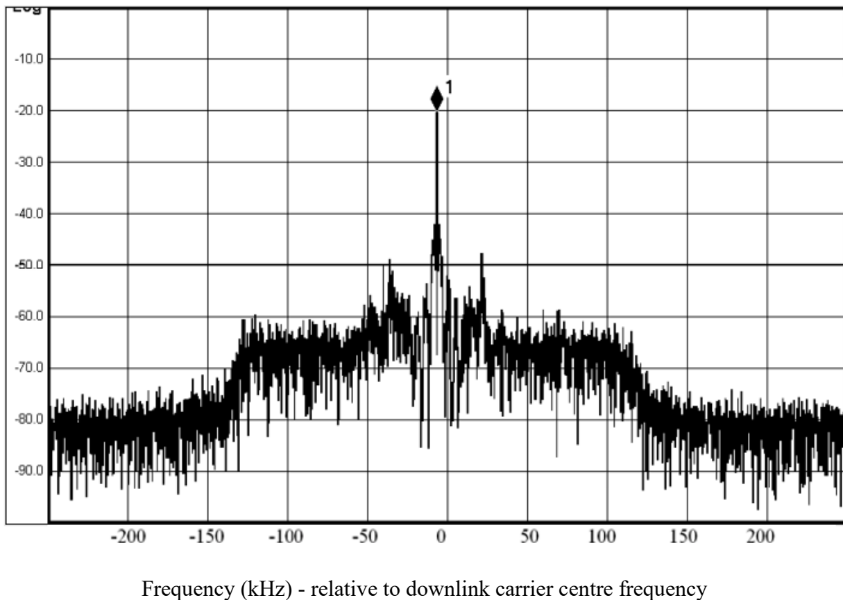
Figure 3-3: Typical Cospas 1544.5 MHz Observed Downlink Signal
