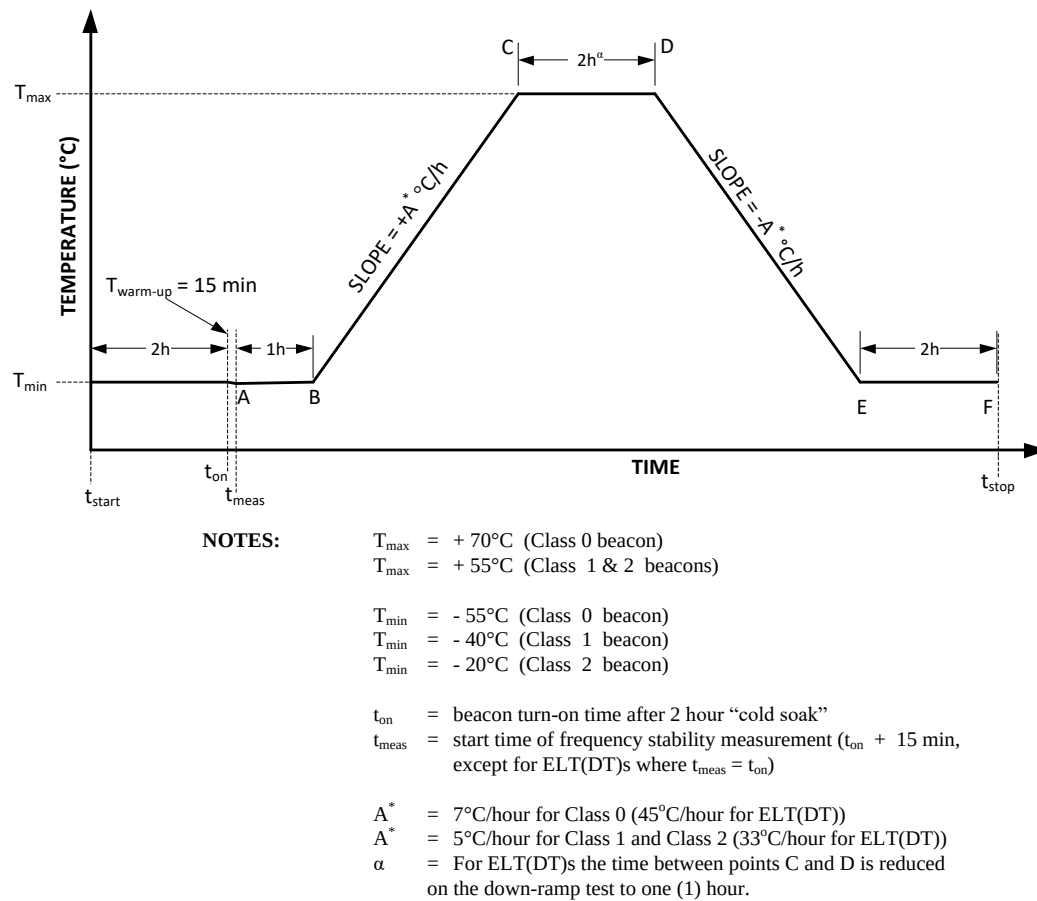
Figure 4.1: Temperature Gradient
