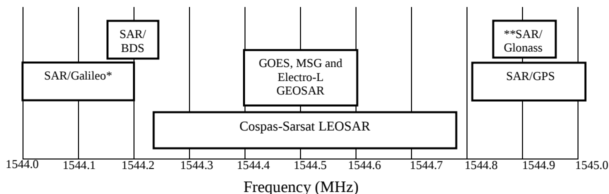
Figure 6.1: 1544 – 1545 MHz Band Plan
