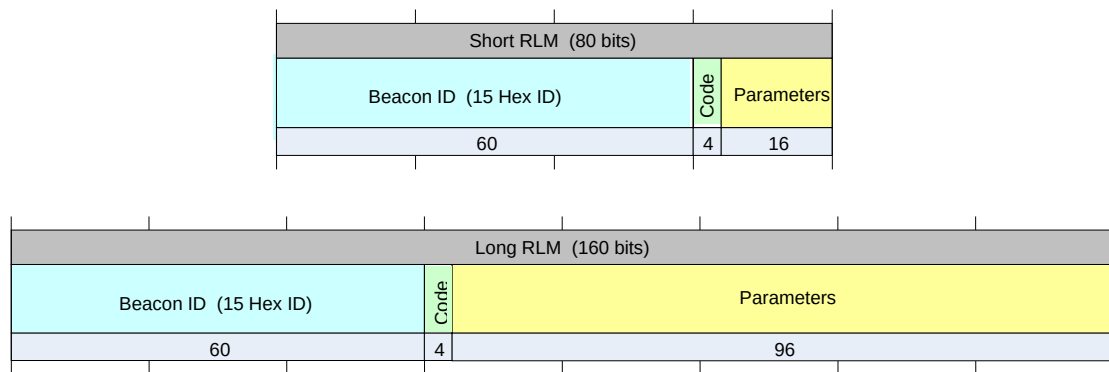
Figure 7.5: Return Link Message Structure
