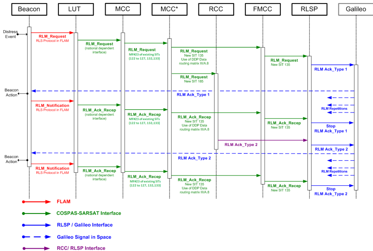
F.7.6.2: RLS data exchange overview for Type 2 Acknowledgment
