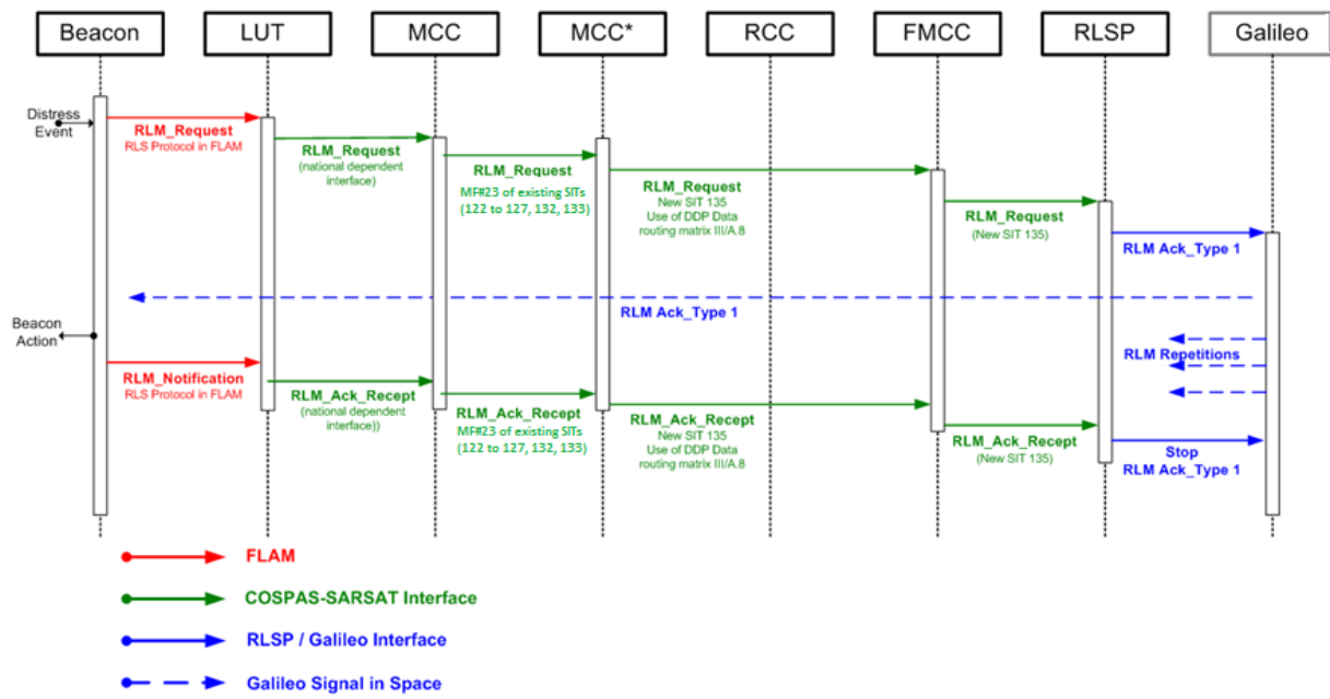
F.7.6.1: RLS data exchange overview for Type 1 Acknowledgment
