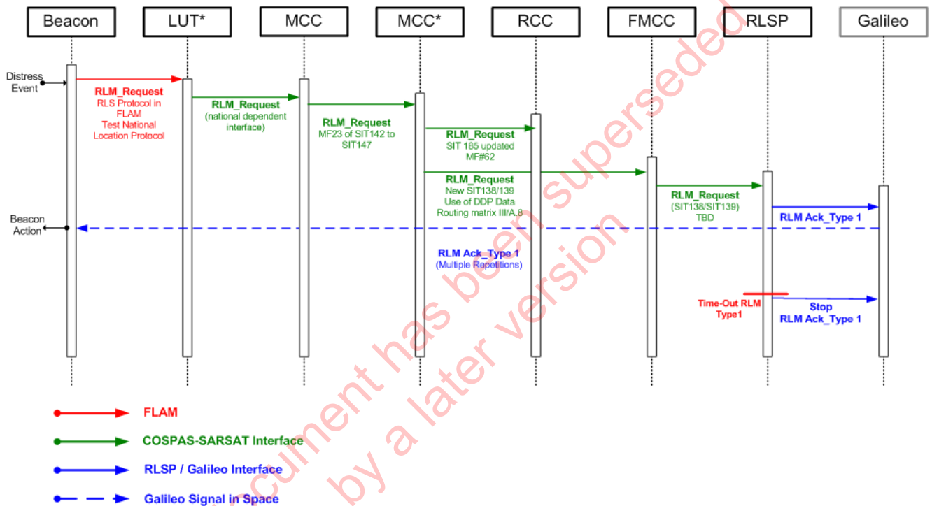
Figure 5.15: High-Level Concept of RLS Process Integration within Cospas-Sarsat
