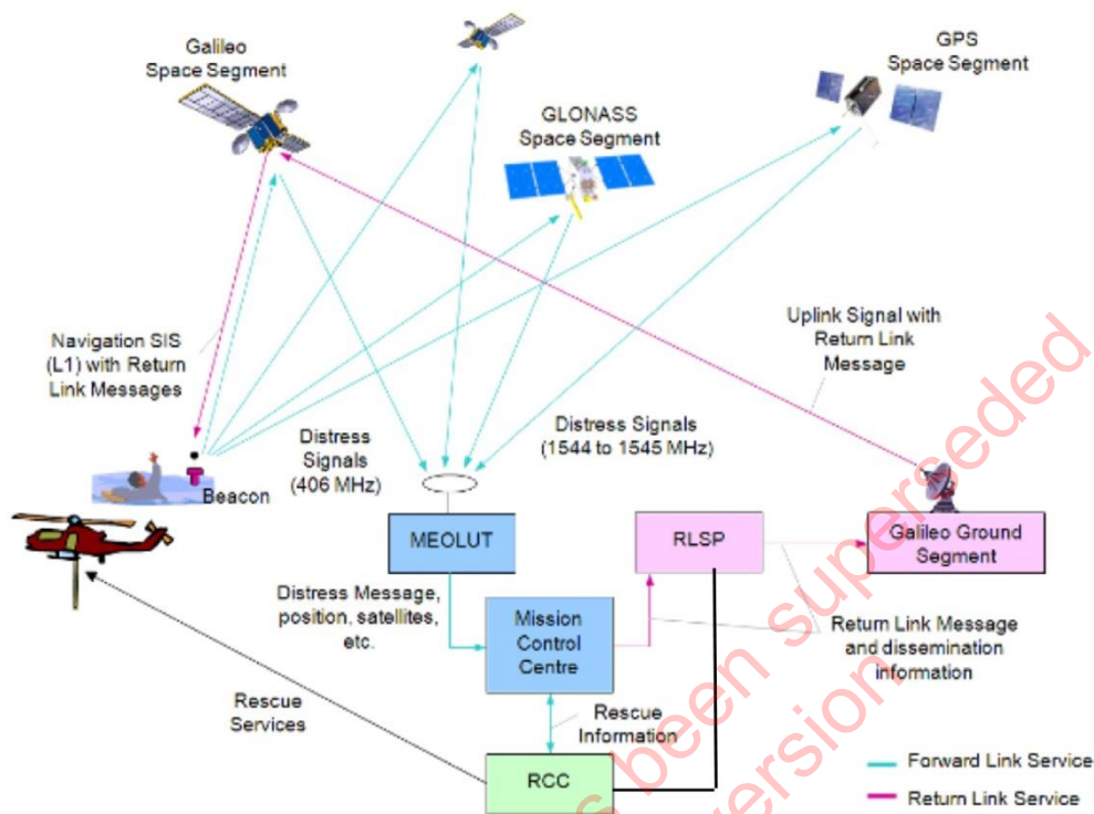
Figure 1.1: The MEOSAR System Concept
