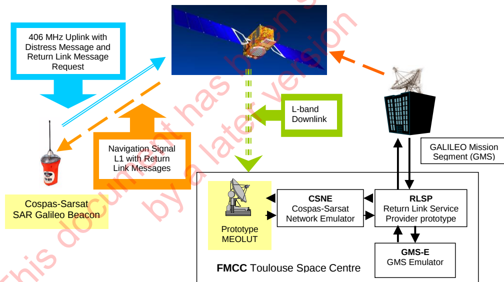
Figure 7.3: Galileo Return Link Service In-Orbit Validation Concept
