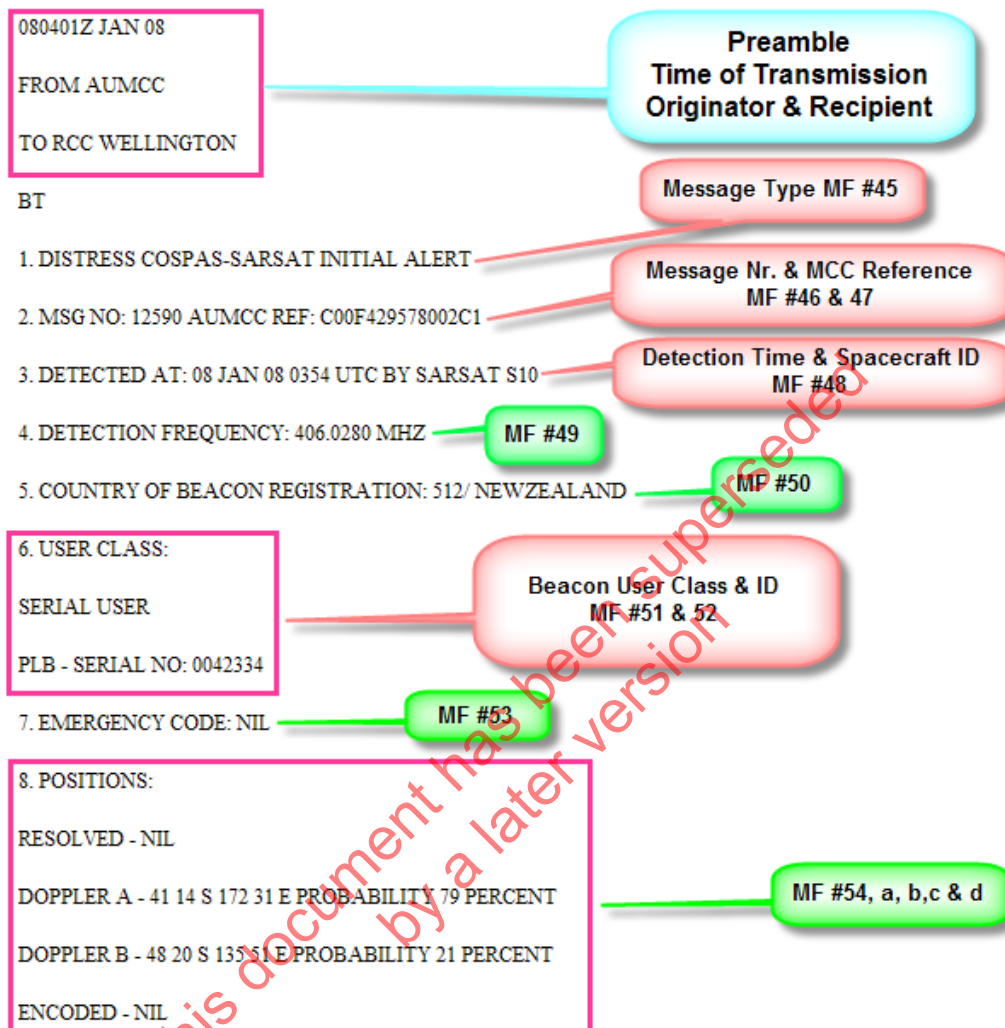
Figure 4.1: Distress Alert Message and Corresponding Message Fields
