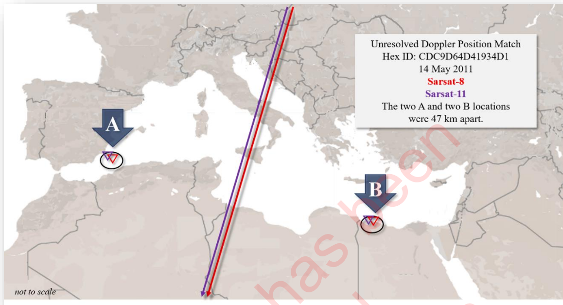
Figure 4.4: Example of an Unresolved Doppler Match
