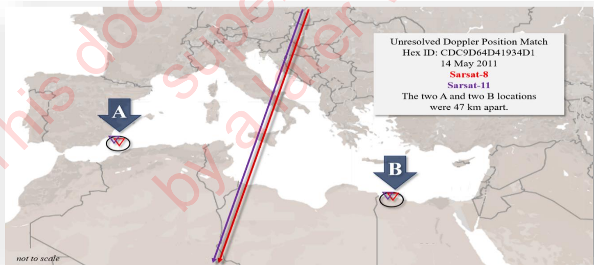
Figure 6.11: Unresolved Doppler Position Match
