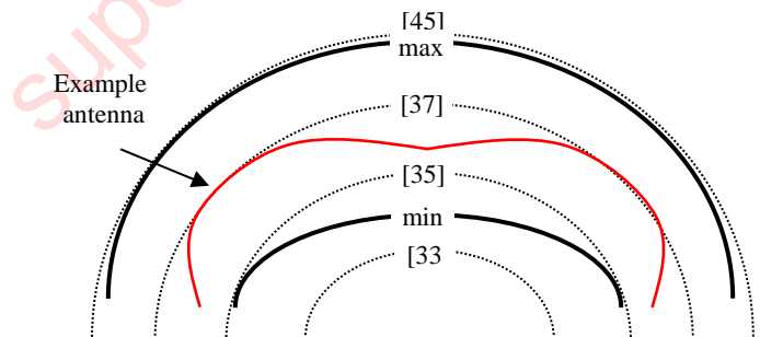
Figure 2-6: Ideal Antenna Pattern
