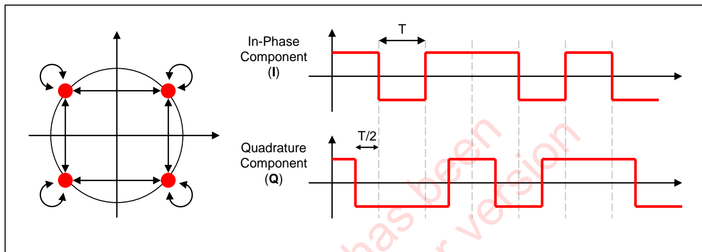
Figure 2-5: OQPSK modulation illustration
