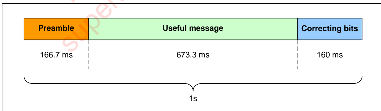
Figure 2-2: Burst general structure
