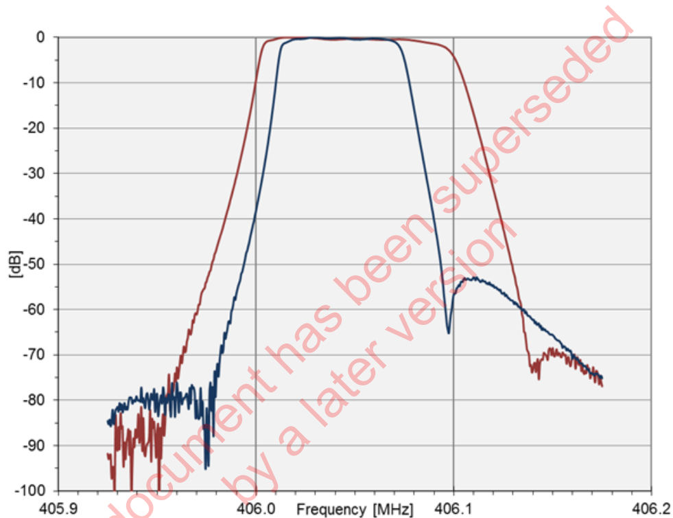
Figure 4.4: Galileo SAR Repeater Normal and Narrow Bandpass Filtering Performance
