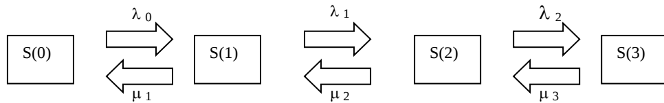
Figure C.8: Diagram of SARP State’s Transitions
