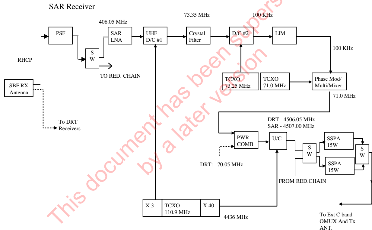
Figure 4.1: INSAT SAR / DRT Repeater Functional Block Diagram
