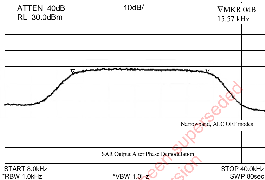
Figure 3.3a: GOES Narrow Band Baseband Spectrum
