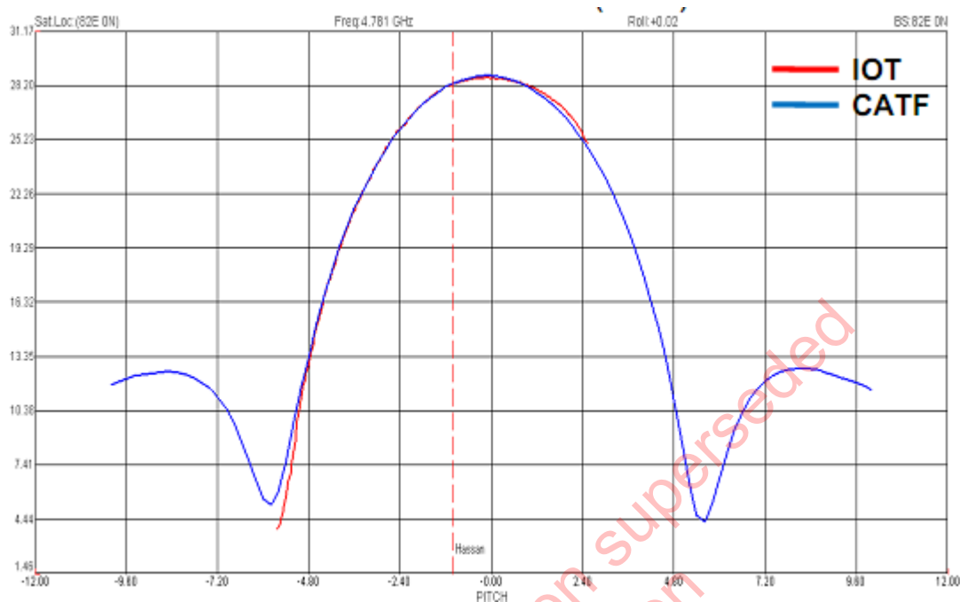
Figure 4.8 Pattern cut at Yaw=0 deg. (Feed 2) with Roll 0 deg.
