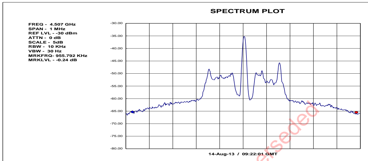
Figure 4.2a: INSAT Transmitter Output Spectral Occupancy With No Test Signal
