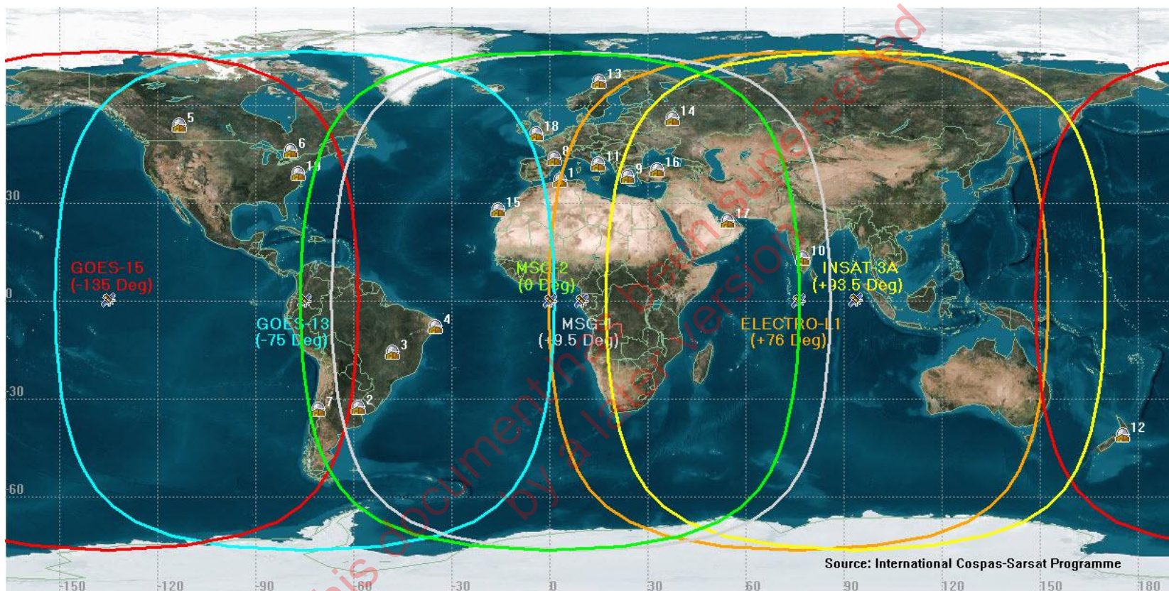
Figure 2.2: Nominal GEOSAR 5 Degree Elevation Contour Coverage (October 2012)
