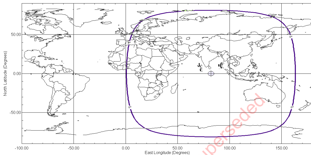
Figure 4-3: INSAT-3D 0-degree Elevation Angle
