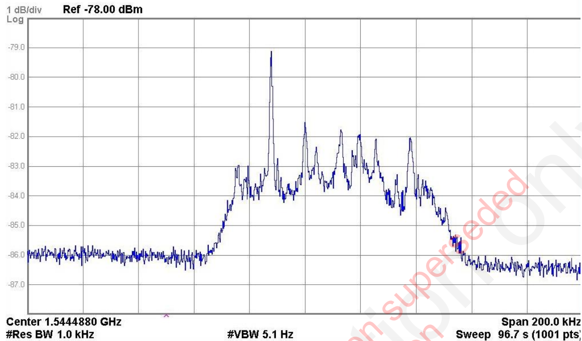
Figure 7-2: Louch-5A Transmitter Spectrum Occupancy
