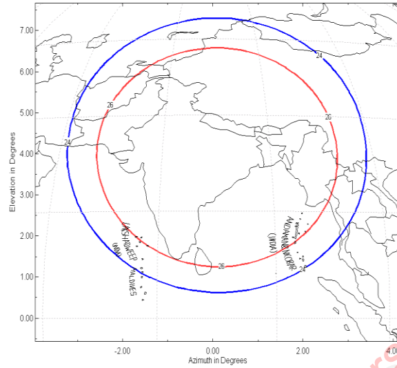
Figure 4-9: INSAT-3D Transmit Antenna Contour Pattern
