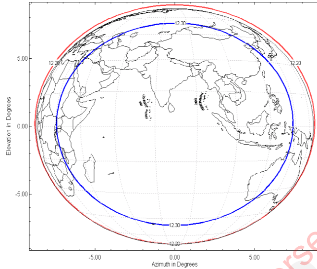
Figure 4-6: INSAT-3D SASR 406.05MHz Receive Antenna Contour Pattern
