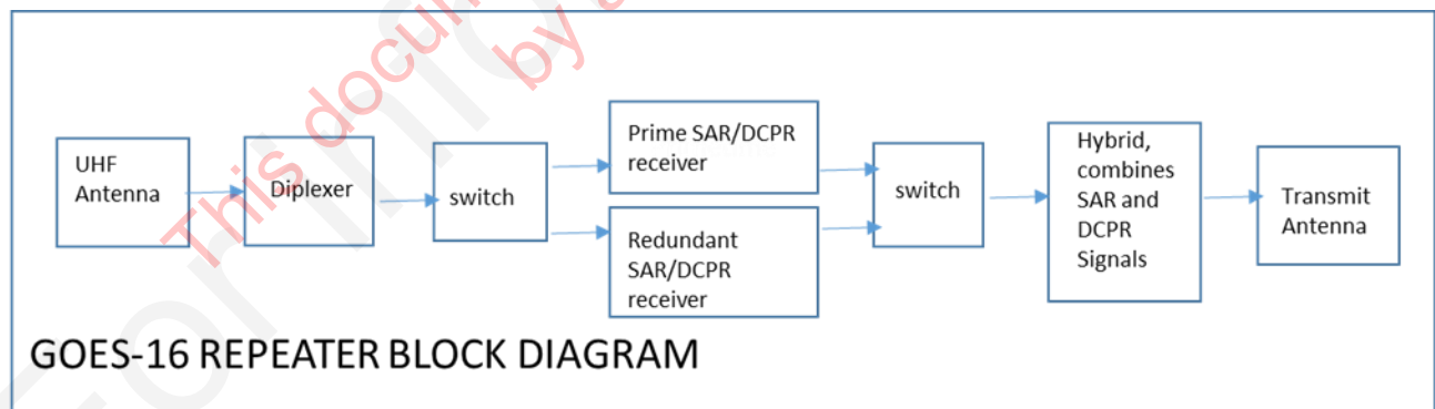
Figure 3-2: GOES-16 repeater block diagram
