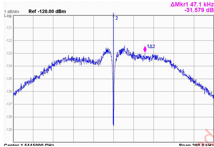
Figure 5-2: Spectrum occupancy of downlink signal in WB mode spanned 300 kHz around 1544.5 MHz
