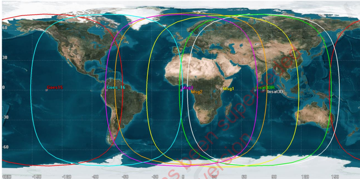
Figure 2-2: Nominal GEOSAR 5 Degree Elevation Contour Coverage (December 2017)
