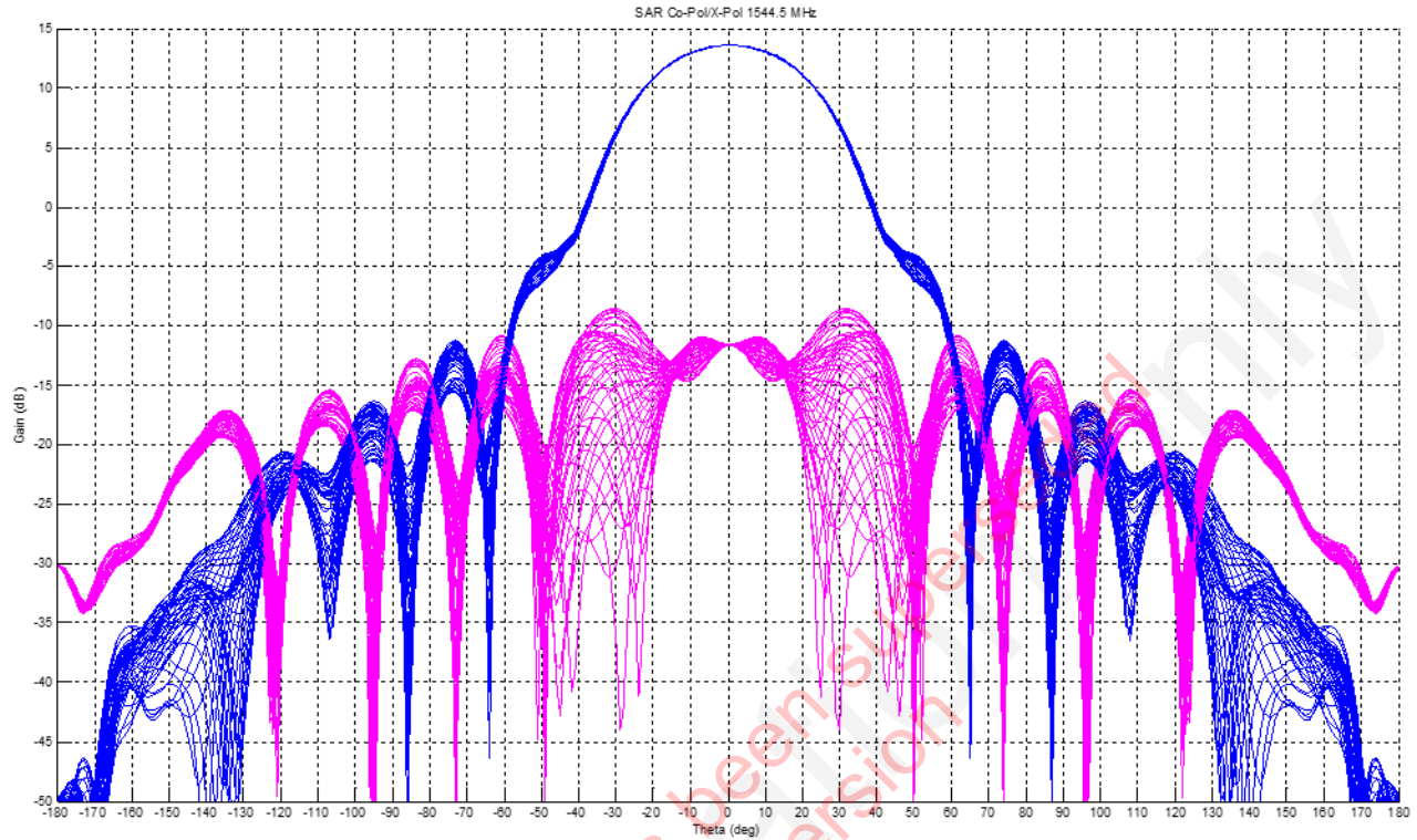
Figure 3-12: GOES-16 SAR Transmit antenna measured at 1544 MHz.
