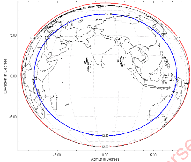
Figure 4.5: INSAT-3D SASR 406.05MHz Receive Antenna Contour Pattern
