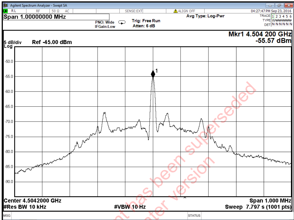
Figure 4.2: INSAT Transmitter Output Spectral Occupancy with No Test Signal
