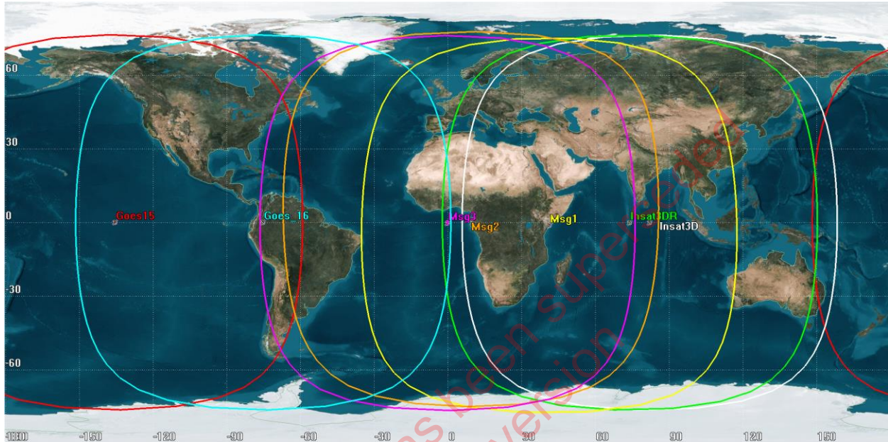
Figure 2.2: Nominal GEOSAR 5 Degree Elevation Contour Coverage (December 2017)
