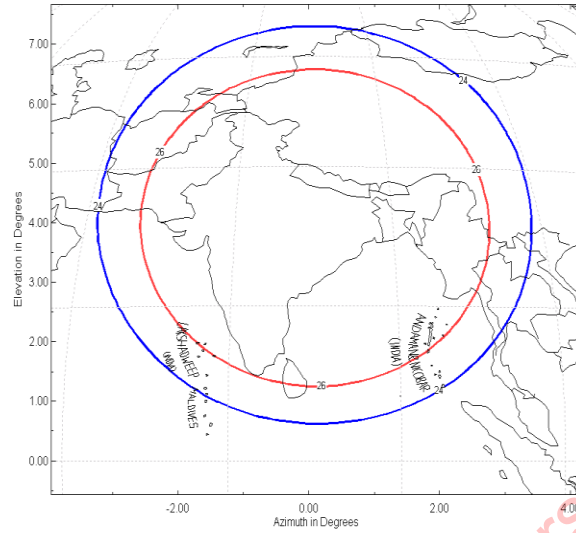
Figure 4.7: INSAT-3D Transmit Antenna Contour Pattern
