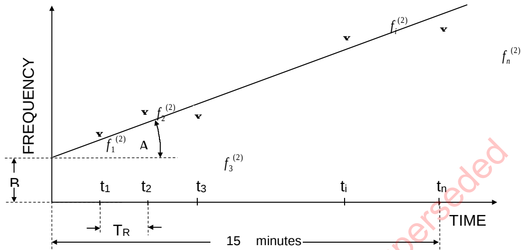
Figure A.4: Medium-Term Frequency Stability Measurement (not to scale)
