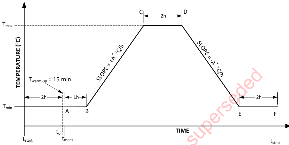
Figure 0.1: Temperature Gradient Test Profile
