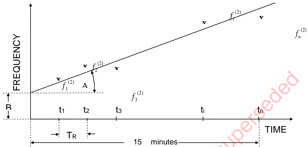
Figure 0.4: Medium-Term Frequency Stability Measurement (not to scale)
