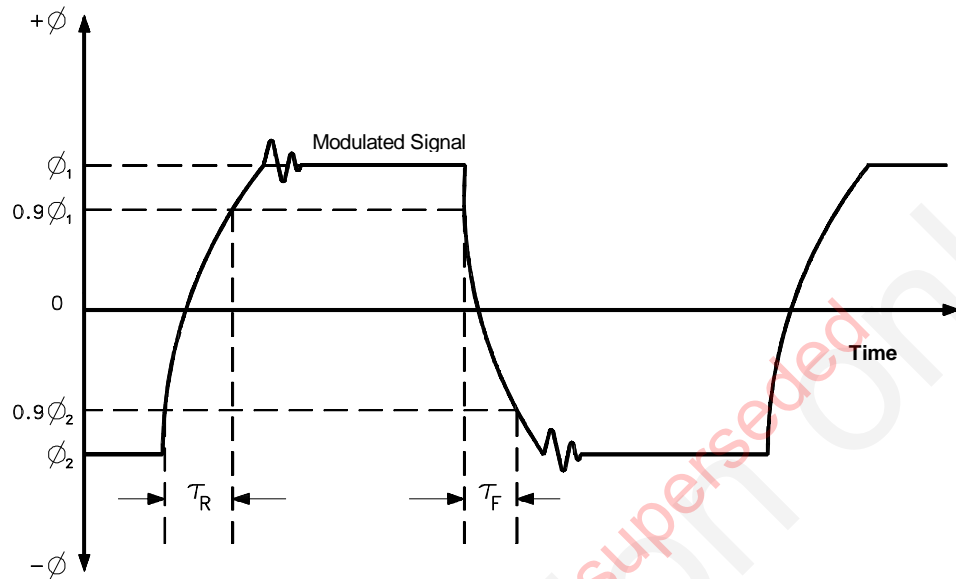
Figure 2.5*: Definition of Modulation Rise and Fall Times
